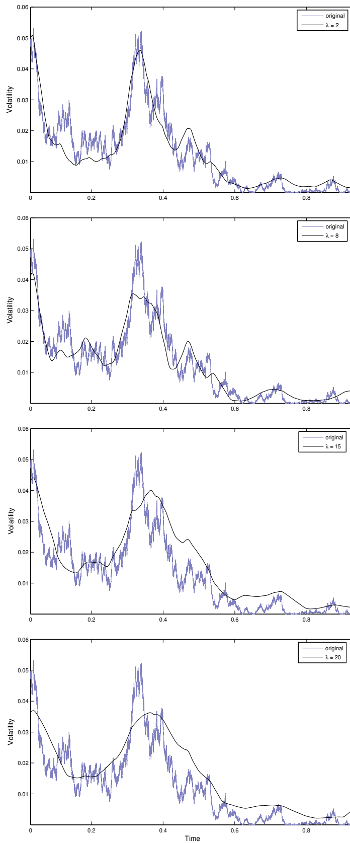
Figure 2.9: Fourier spot volatility estimation with unevenly sampled data and high microstructure noise.
