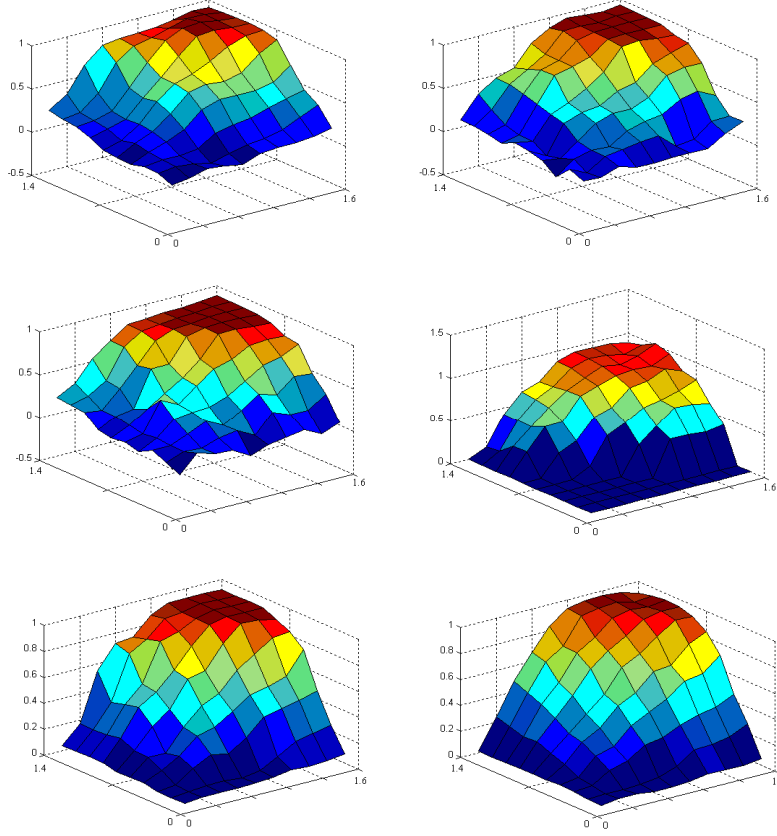
Figure III.23: Surface mapping of ANN performance for z=\sin(x*y) ; (top left) experiment 1, (top right) experiment 2, (middle left) experiment 3, (middle right) experiment 4, (bottom left) experiment 5, (bottom right) experiment 6.
