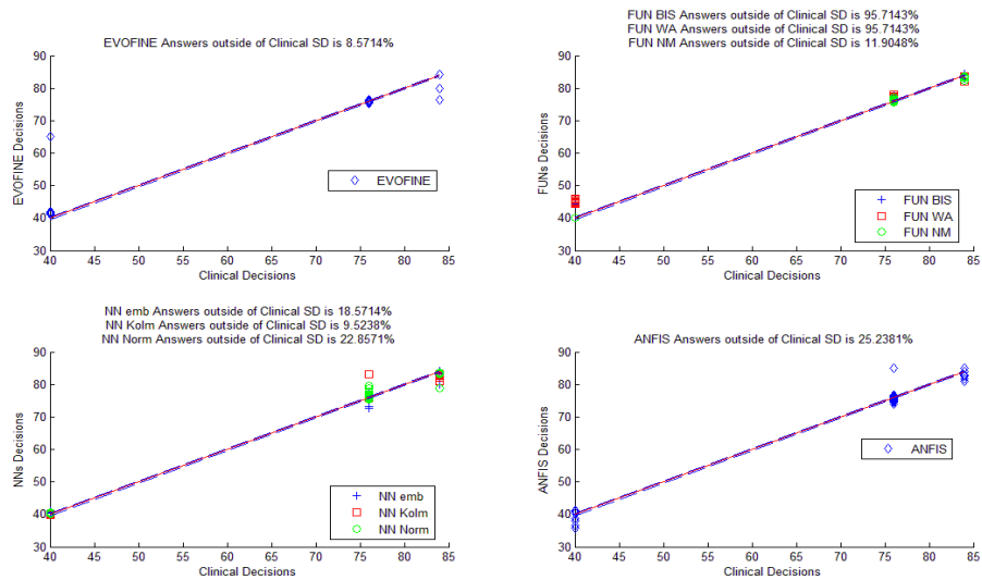
Figure 6.54: Scatter diagram of models' vs. clinical decisions for Pmax COPD
