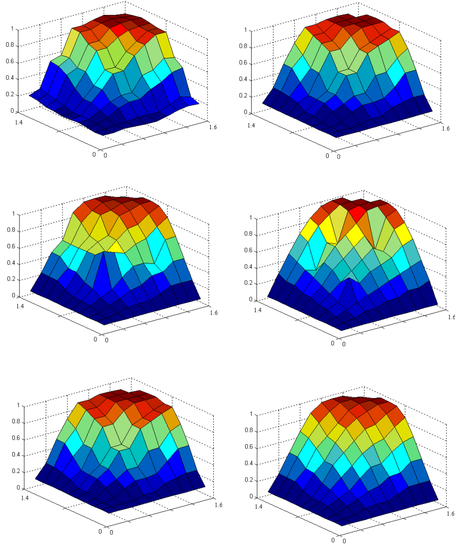
Figure III.18: Surface mapping of FUN performance for z=\sin(x*y) ; (top left) experiment 1, (top right) experiment 8, (middle left) experiment 10, (middle right) experiment 11, (bottom left) experiment 12, (bottom right) experiment 20.
