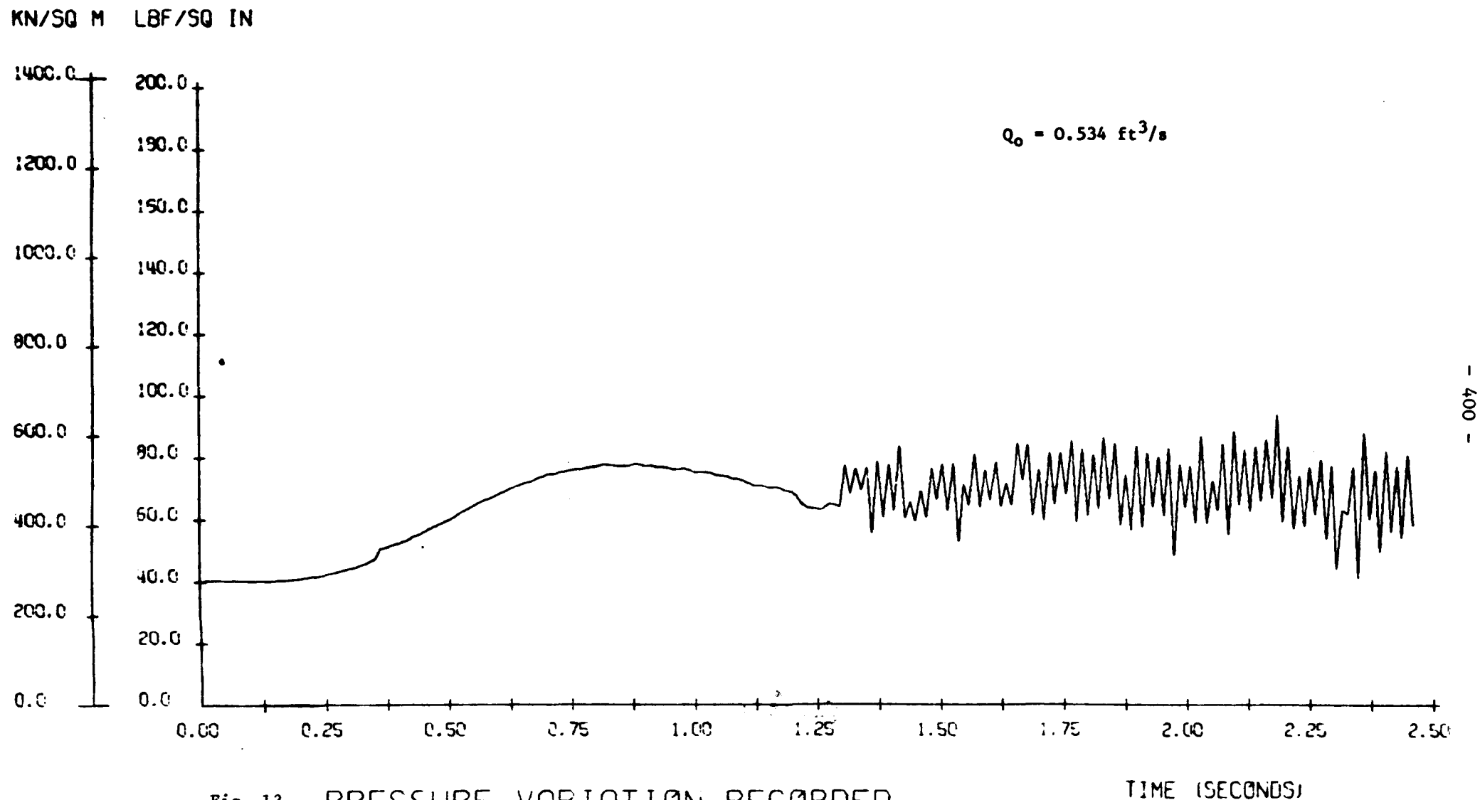
Fig. 13 PRESSURE VARIATION RECORDED AT TANK 6 DURING TEST CASE 1
