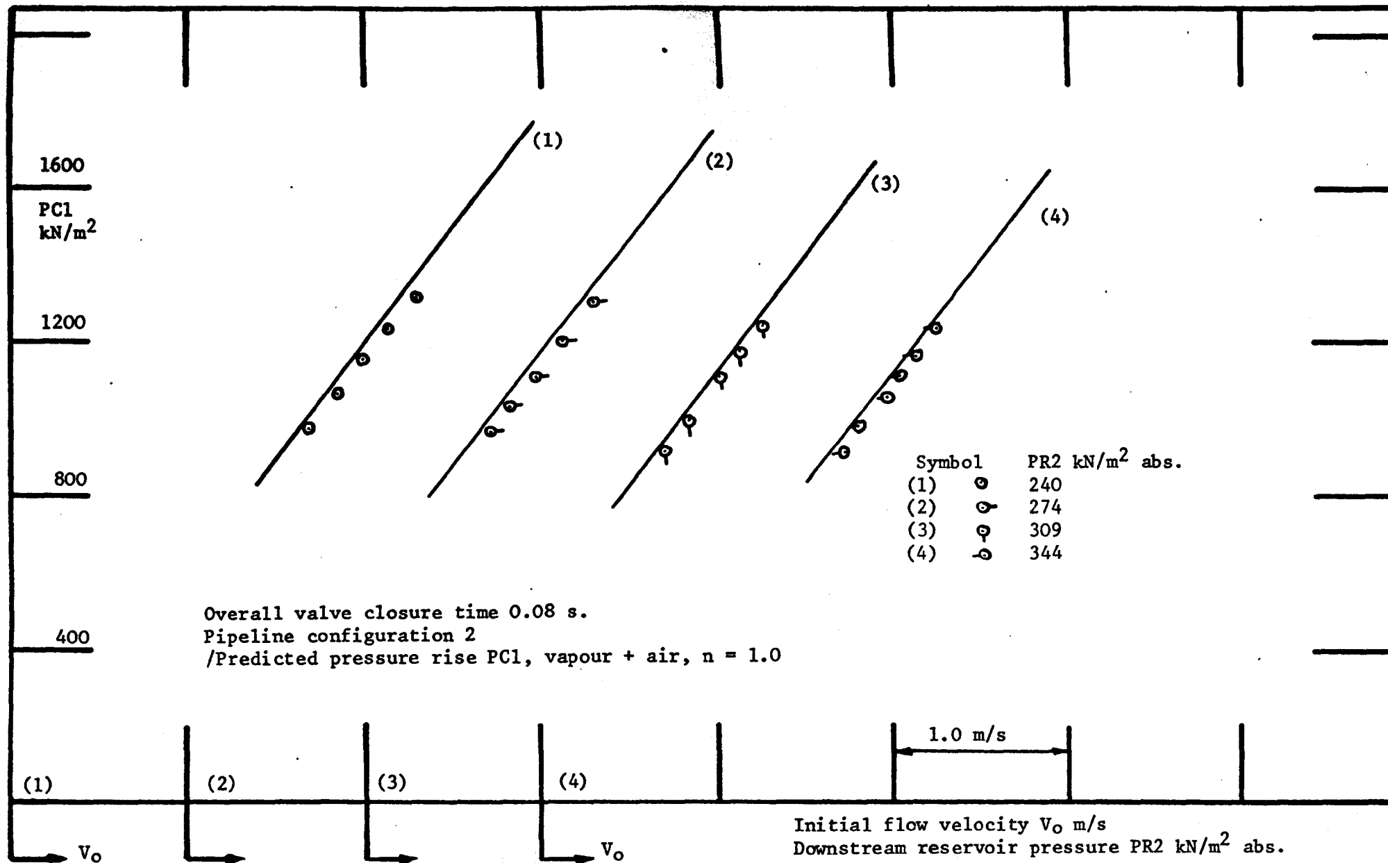
Fig. 92 Pressure rise ( PC1 ) above steady state, on the downstream face of the valve following the collapse of the first vapour cavity, for a range of initial flow velocities ( V_0 ) and downstream reservoir pressures ( PR2 ).
