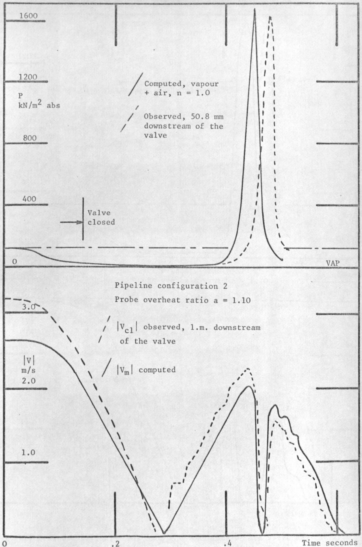
Fig.120 Pressure and velocity variations downstream of the valve during and following valve closure and the growth and collapse of the first cavity. Initial conditions, V_0 = 2.67 m/s, PR2 = 120 \text{kN/m}^2 abs, TC = 0.14 s.
