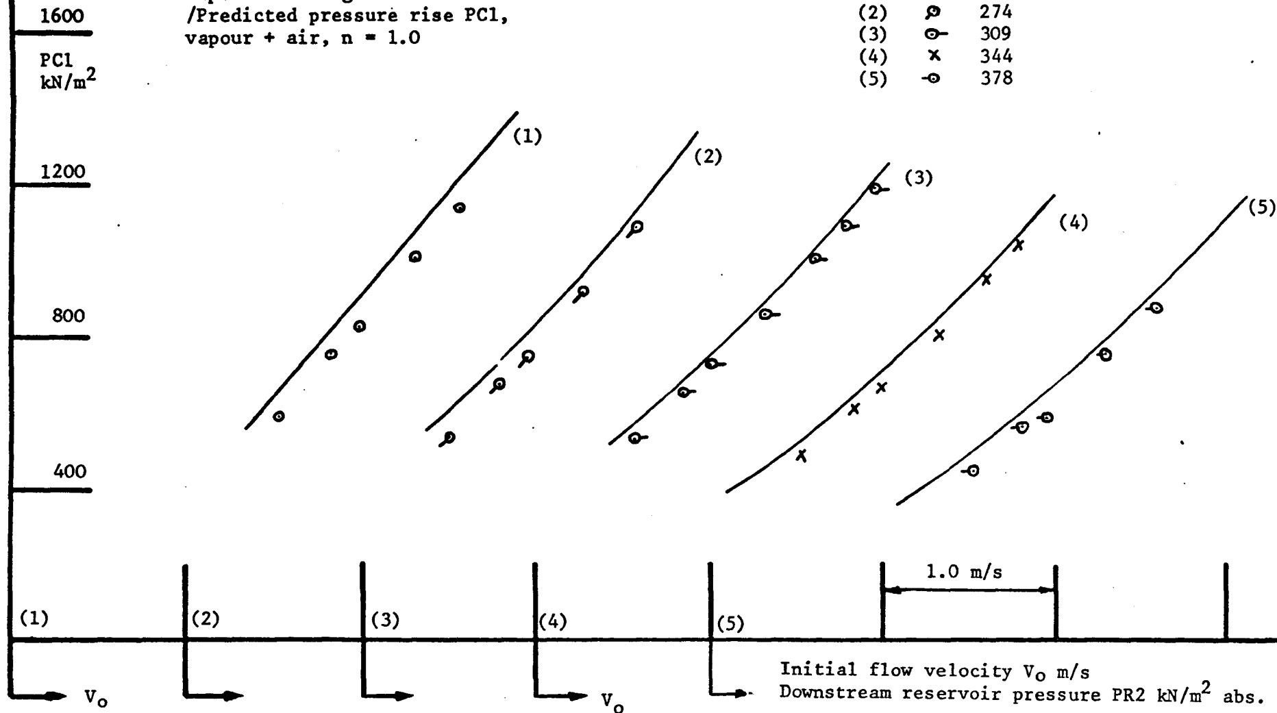
Fig. 93 Pressure rise PC1 , above steady state, on the downstream face of the valve following the collapse of the first cavity, for a range of initial flow velocities ( V_0 ) and downstream reservoir pressures (PR2).
