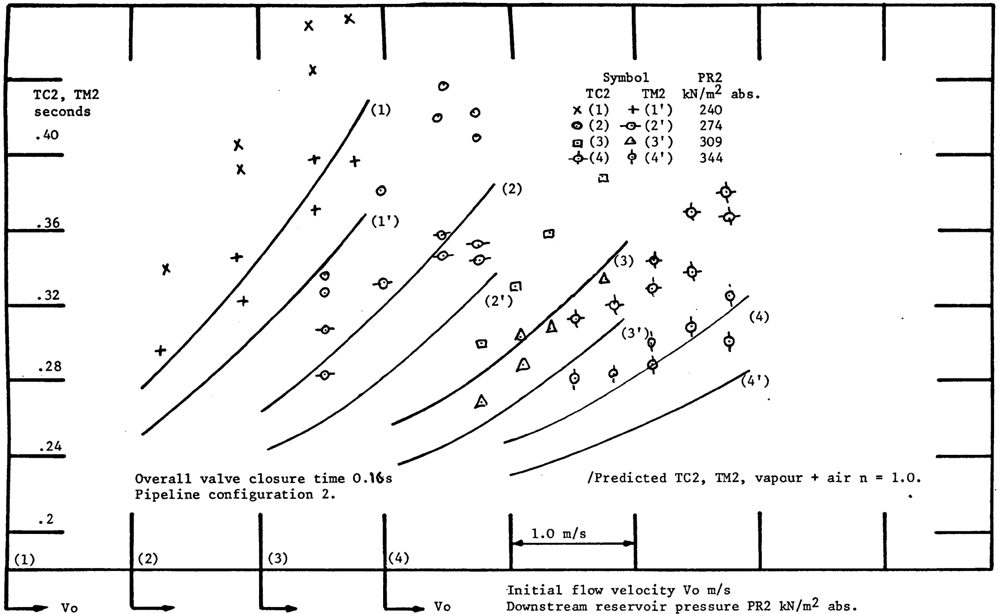
Fig. 116 Time to minimum pressure (TM2) and subsequent cavity collapse (TC2) for the second cavity formed downstream of the valve for a range of initial flow velocities ( V_0 ) and downstream reservoir pressures (PR2).
