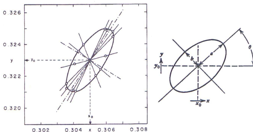
Figure 1.21: (A) An example of the experimental results obtained by MacAdam showing the standard deviations involved in colour matching a fixed chromaticity (x_0, y_0) along different direction in the 1931 CIE- x, y chromaticity space. (B) Illustration of ellipse parameters; (x_0, y_0) = coordinates of centre, a =major semiaxis, b =minor semiaxis, \theta =angle in degrees. Reproduced from Wyszecki and Stiles (1982).
