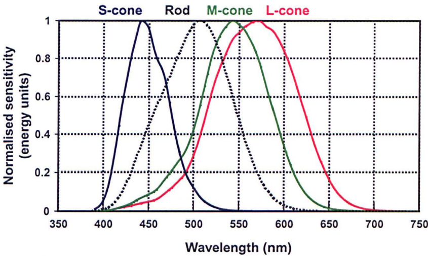
Figure 1.11: Stockman and Sharpe (2000) cone fundamentals. The curves represent normalised spectral sensitivity of the four receptor types in the human retina (Stockman et al. 1999; Stockman and Sharpe 2000). Data obtained from cvrl website (Color vision research laboratories) http://www-cvrl.ucsd.edu/ .
