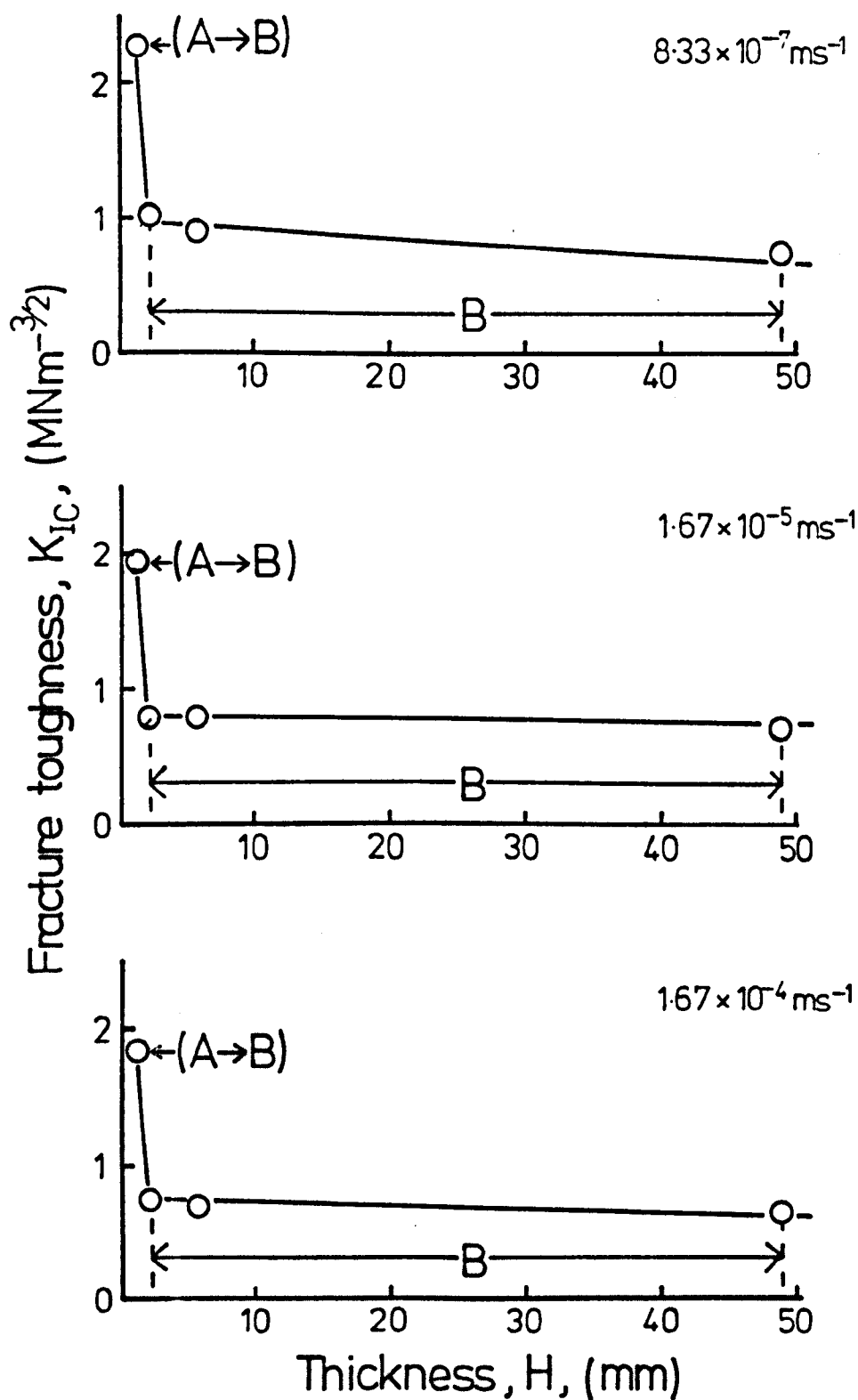
Figure 7.13 Fracture toughness, K_{IC} , versus specimen thickness, H . Unmodified epoxy. 20^\circ\text{C}
