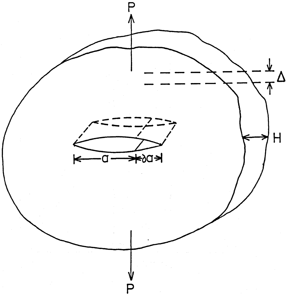
Figure 3.1 Loading of a cracked elastic body.
