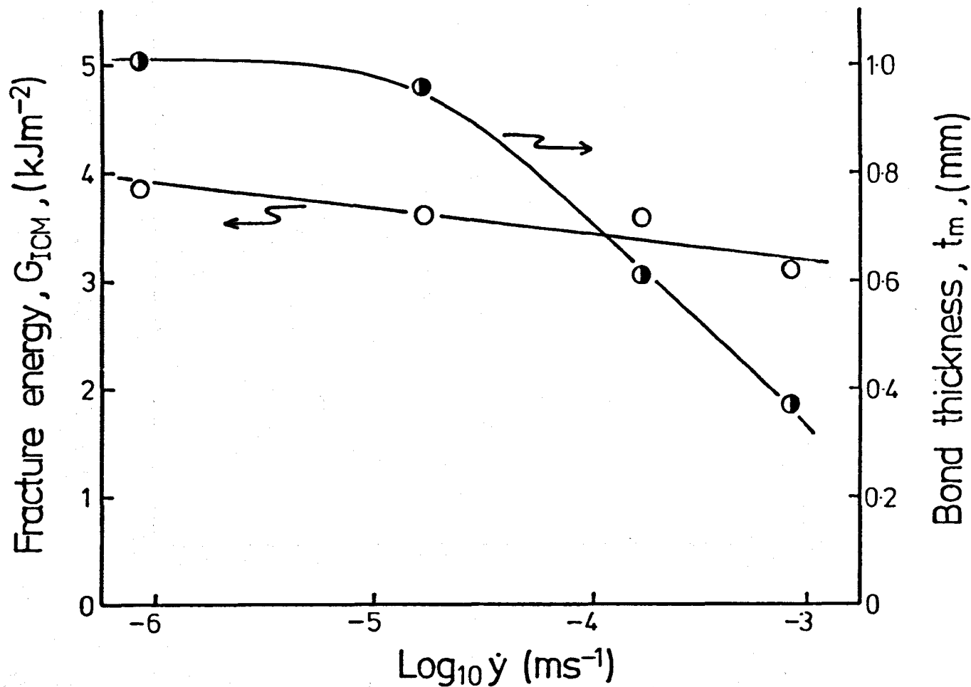
Figure 10.4 Adhesive fracture energy maximum, G_{\text{ICM}} , and corresponding bond thickness, t_m , versus displacement rate, \dot{\gamma} . 20°C.
