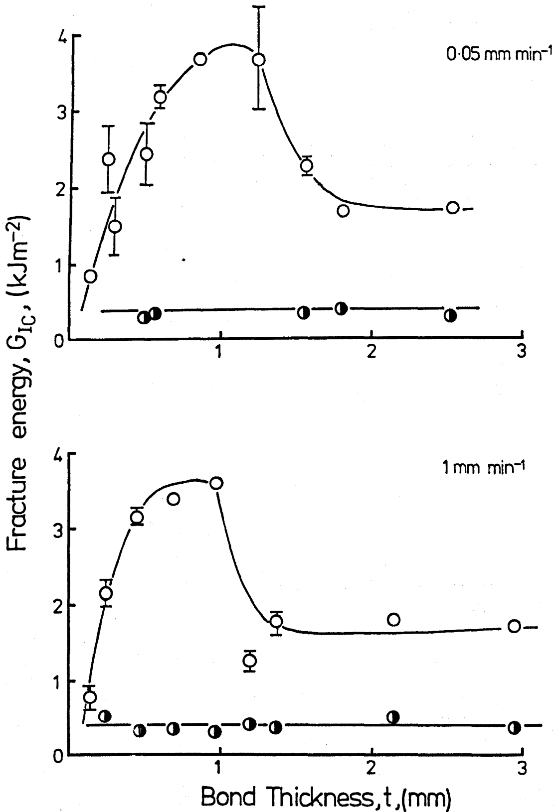
Figure 8.7 Adhesive fracture energy, G_{IC} , versus bond thickness, t , for various displacement rates. 20^{\circ}\text{C} , 12mm joint width. -o- stable or initiation, -●- arrest.
