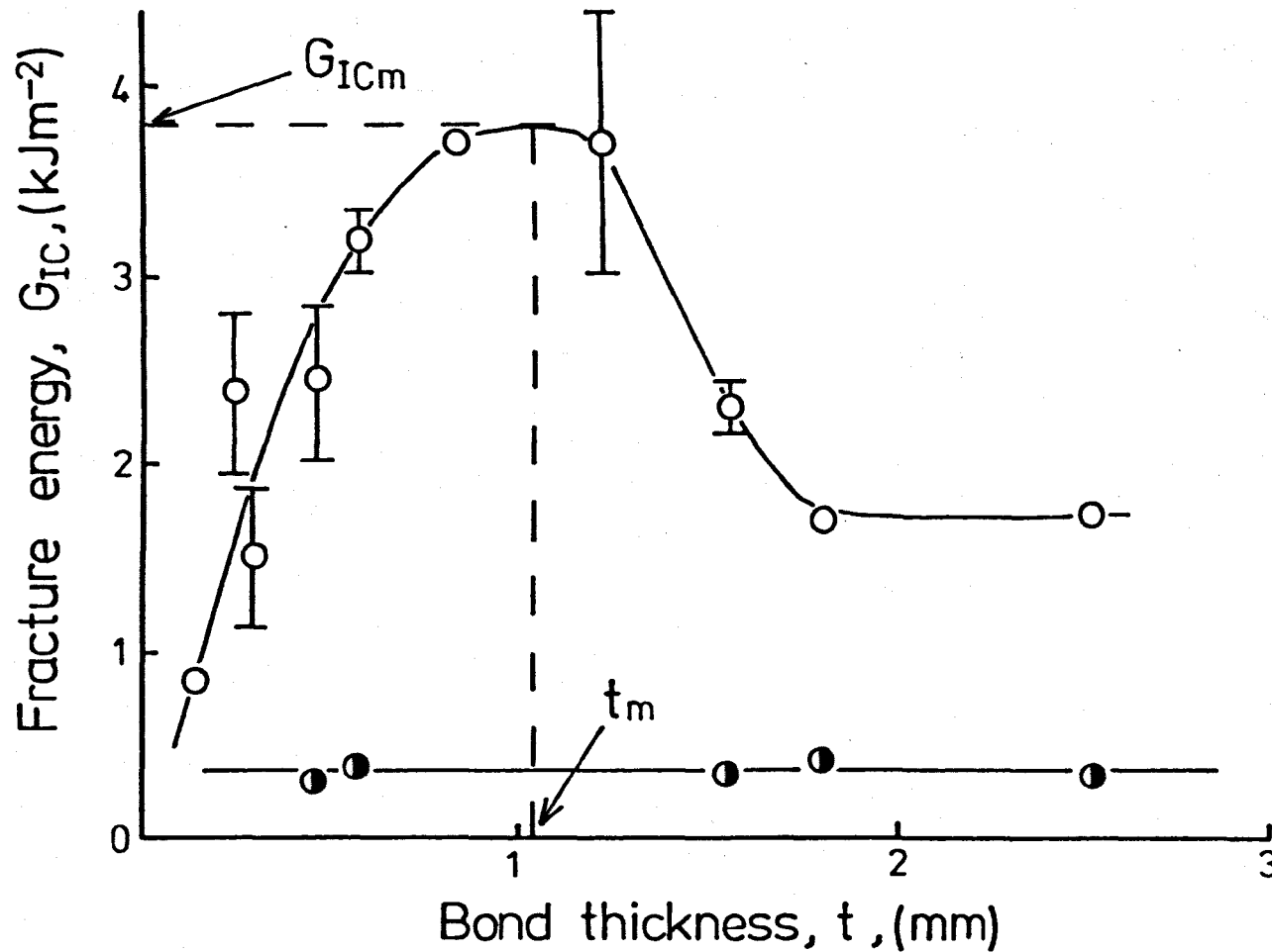
Figure 8.1 Adhesive fracture energy, G_{IC} , versus bond thickness, t . 0.05 \text{ mm min}^{-1} displacement rate, 20^\circ\text{C} . —○— stable or initiation, —●— arrest.
