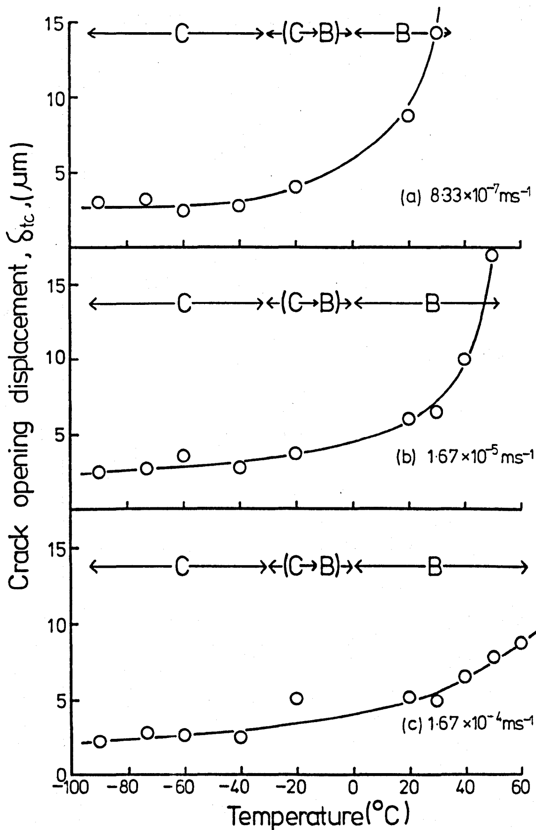
Figure 9.1 Critical crack opening displacement, \delta_{tc} , versus temperature. Unmodified epoxy.
