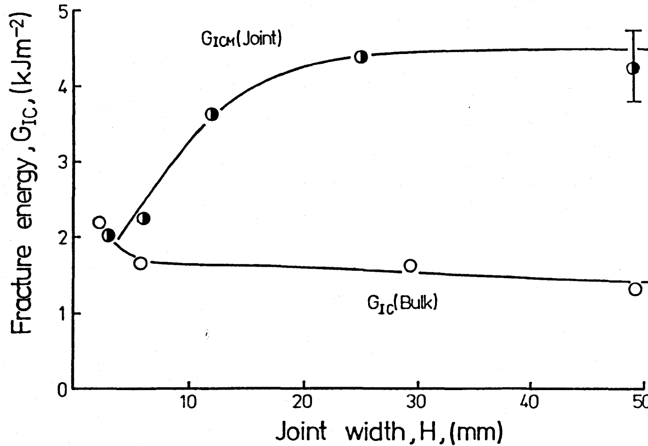
Figure 10.8 Fracture energy, G_{IC} (joint), and G_{IC} (bulk) versus joint width, H . Rate: 1 \text{ mm min}^{-1} . 20^\circ\text{C} .
