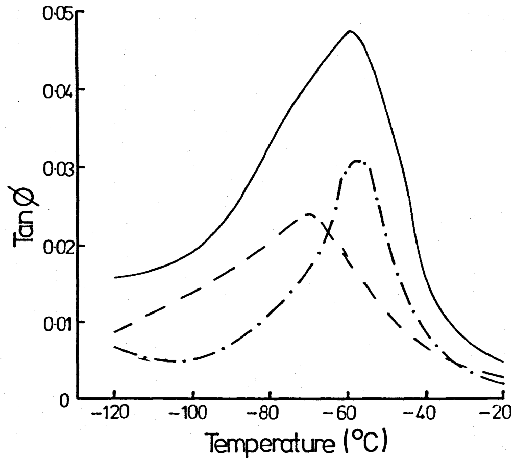
Figure 7.6 Loss factor, \tan \delta , as a function of temperature, -120^{\circ}\text{C} to -20^{\circ}\text{C} . — Rubber-modified epoxy, — — — Unmodified epoxy, — · — · — \Delta \tan \delta .
