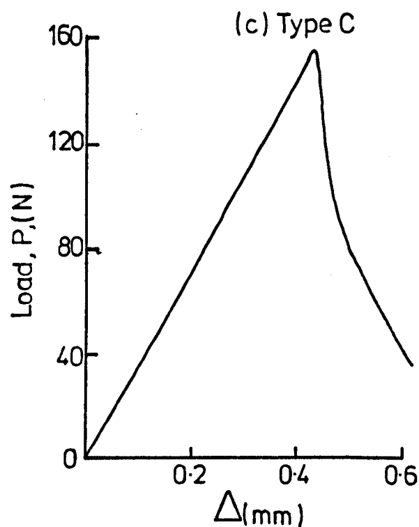
Figure 7.7 Typical load versus displacement curves obtained from 5.8mm thick compact tension specimens.
