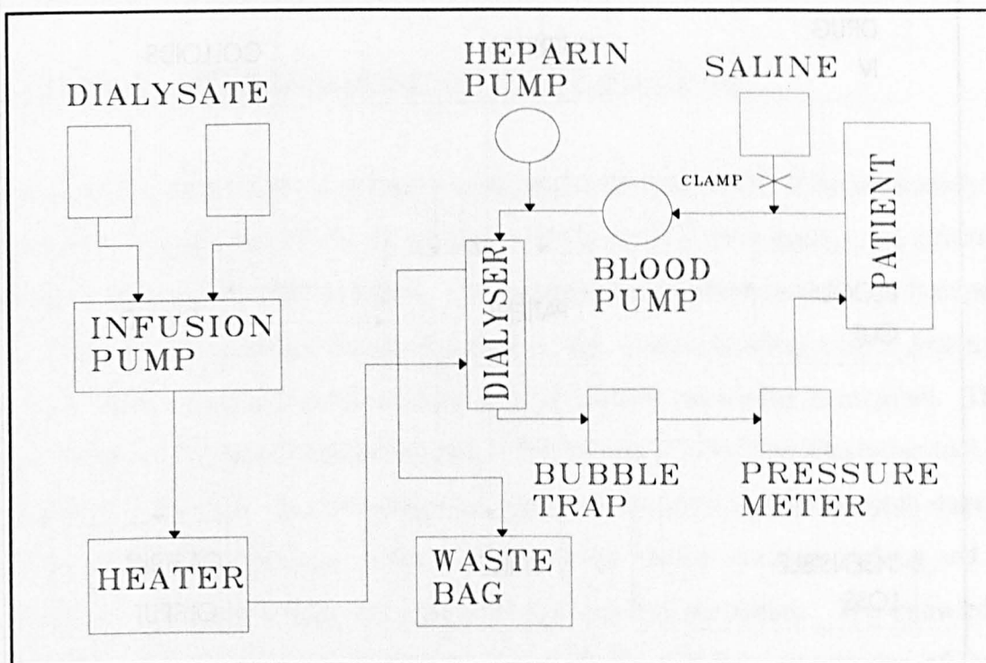
Figure 5.19 Continuous venovenous haemodialysis schematic
