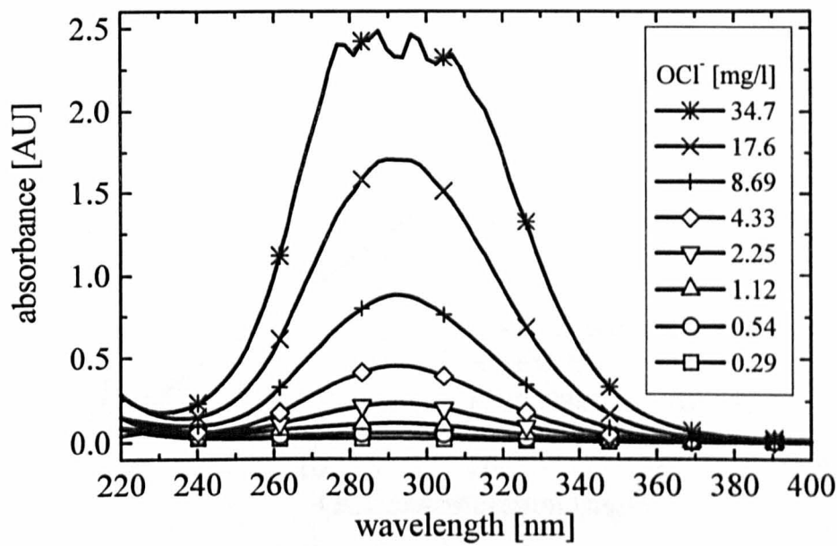
Fig. 5-14: Absorption measurements from 220 nm up to 400 nm of \text{OCl}^- at several concentrations smaller than 35 mg l -1 (pH = 10.2, \Theta = 17.5 °C, Z_{\text{LCW}} = 203 mm)
