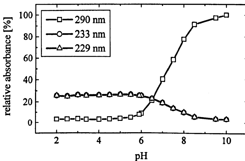
Fig. 5-7: Relative absorbance of the free chlorine species Cl 2 at 229 nm, HOCl at 233 nm and OCl - at 290 nm as a function of pH.
