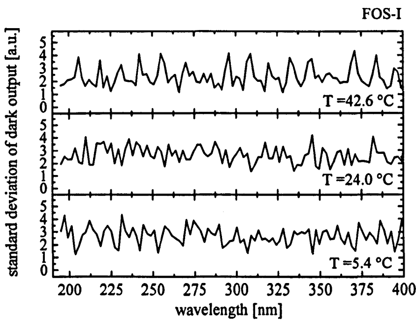
Fig. 3-3: Standard deviation of the dark output of FOS-I at an integration time of 585 ms as a function of wavelength at 42.6 °C, 24.0 °C and 5.4 °C.
