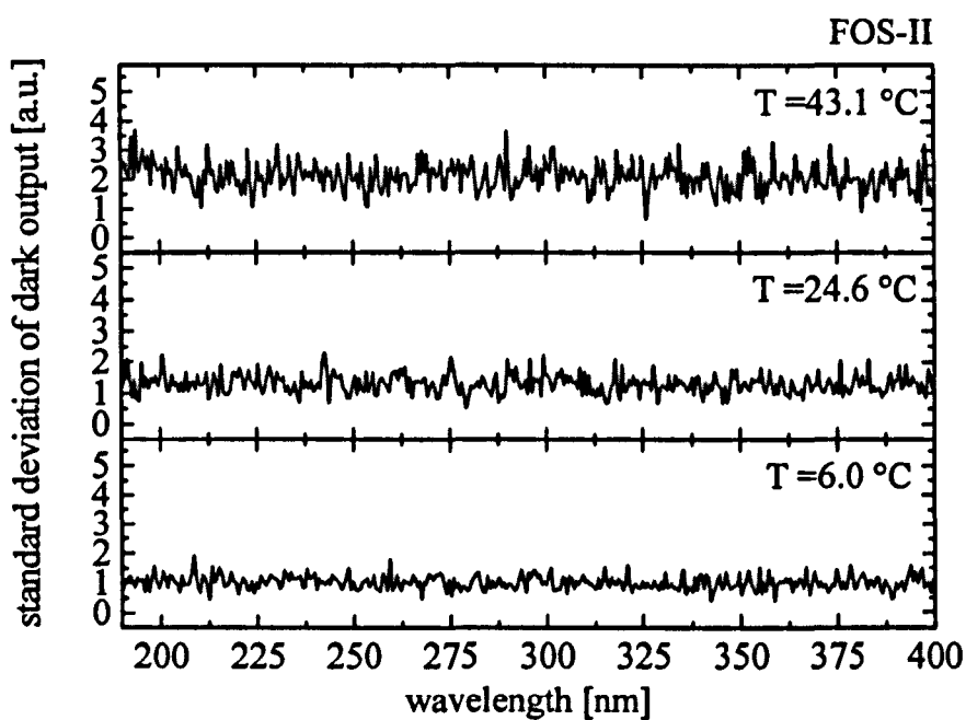
Fig. 3-4: Standard deviation of the dark output of FOS-II at an integration time of 585 ms as a function of wavelength at 43.1 ^{\circ}\text{C} , 24.6 ^{\circ}\text{C} and 6.0 ^{\circ}\text{C} .
