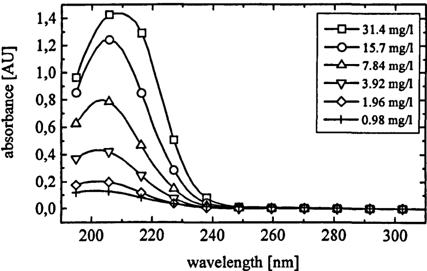
Fig. 4-7: Nitrate ( \text{NO}_3^- ) absorption measured with reflectance cell having an optical pathlength of 10 mm, containing 31.4, 15.7, 7.8, 3.9, 2.0 and 1.0 mg l -1 \text{NO}_3^- in de-ionized water.
