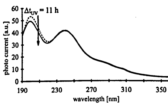
Fig. 2-5: Spectral output power of a UV-improved fibre before (dashed line) and after (solid line) 11 h of UV-light irradiation.
