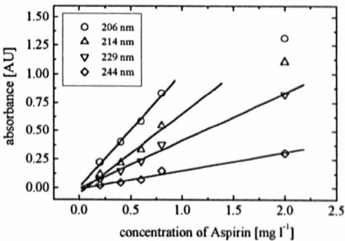
Fig. 5-17: Calibration curves of Aspirin (206 nm, 214 nm, 229 nm and 244 nm).
