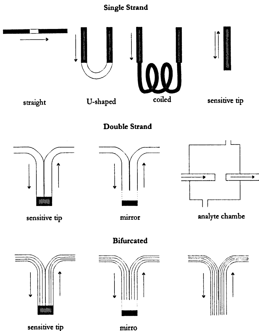
Fig. 1-1: Different types of fibre-optic based sensor cells.
