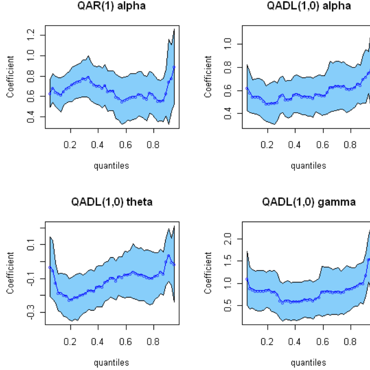
Figure 3: Coefficient estimates
