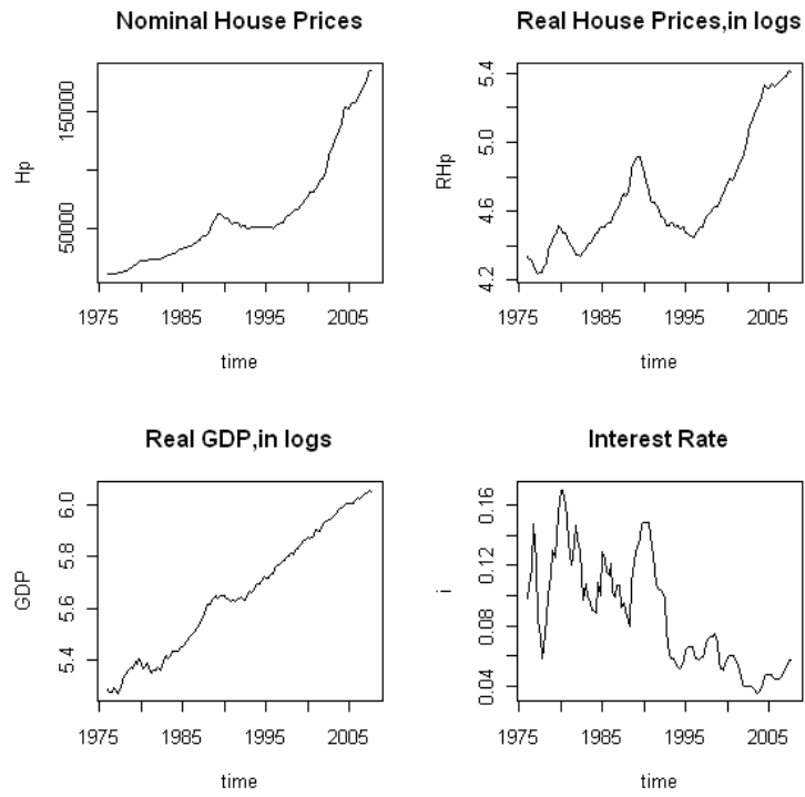
Figure 1: Time Series
