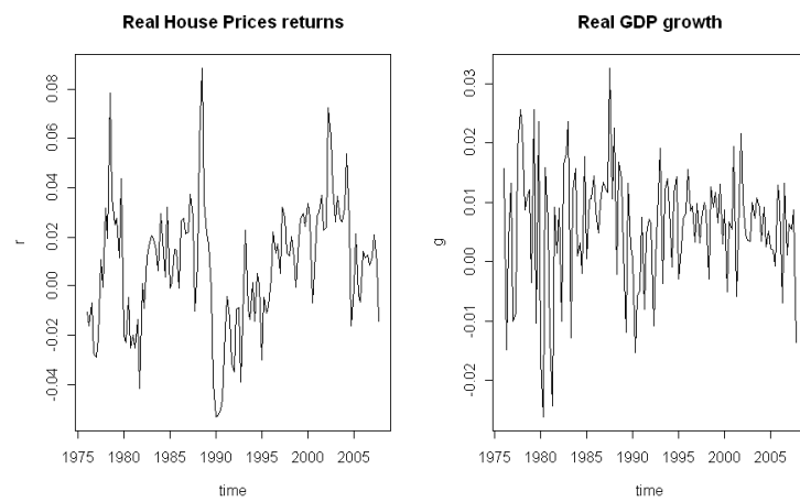
Figure 2: Time Series
