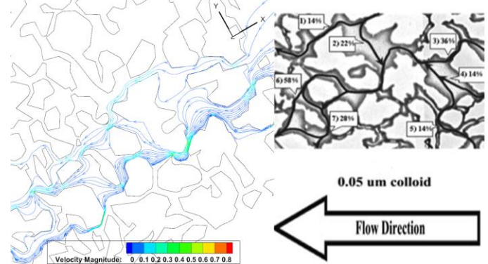
Figure 5: (a) Stream lines distribution with velocity vectors. Higher velocities are calculated at the upper part of the grain (b) Experimental results from Sirivithayapakorn el. al. (21) showing massless particle trajectory (thick black line)
