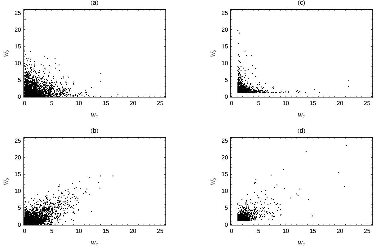
Fig. 3. (a) simulated i.i.d. \text{Exp}(0.5) losses; (b) simulated dependent losses following C^{\text{RCl}}(u_1, u_2; 1) with \text{Exp}(0.5) marginals; (c) simulated i.i.d. \text{Pareto}(2.41, 1.17) losses; (d) simulated dependent losses following C^{\text{RCl}}(u_1, u_2; 1) with \text{Pareto}(2.41, 1.17) marginals.
