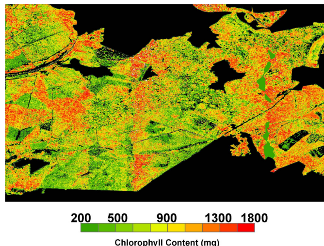
Figure 4. Chlorophyll content map of the study area derived from CASI data and ground data of chlorophyll content. Areas in black represent missing data or non-vegetated areas.
