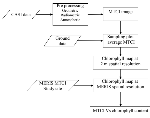
Figure 2. Methodology for MTCI validation.
