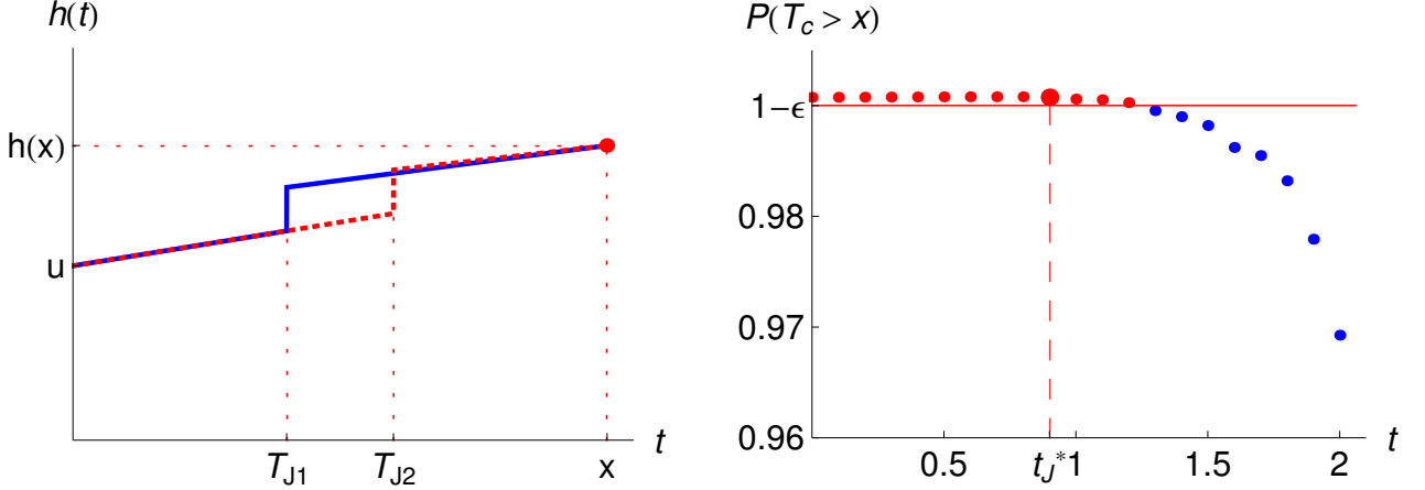
Figure 9: Left panel: two possible candidates h_1(t), h_2(t) \in \mathcal{H} . Right panel: P(T > x) as a function of the location t_J of the jump of size J . Parameter values: \lambda = 5 , \alpha = 0.1 , u = 12.5 , c_1 = 3 , x = 2 , J = 2.5 and \epsilon = 0.01 .
