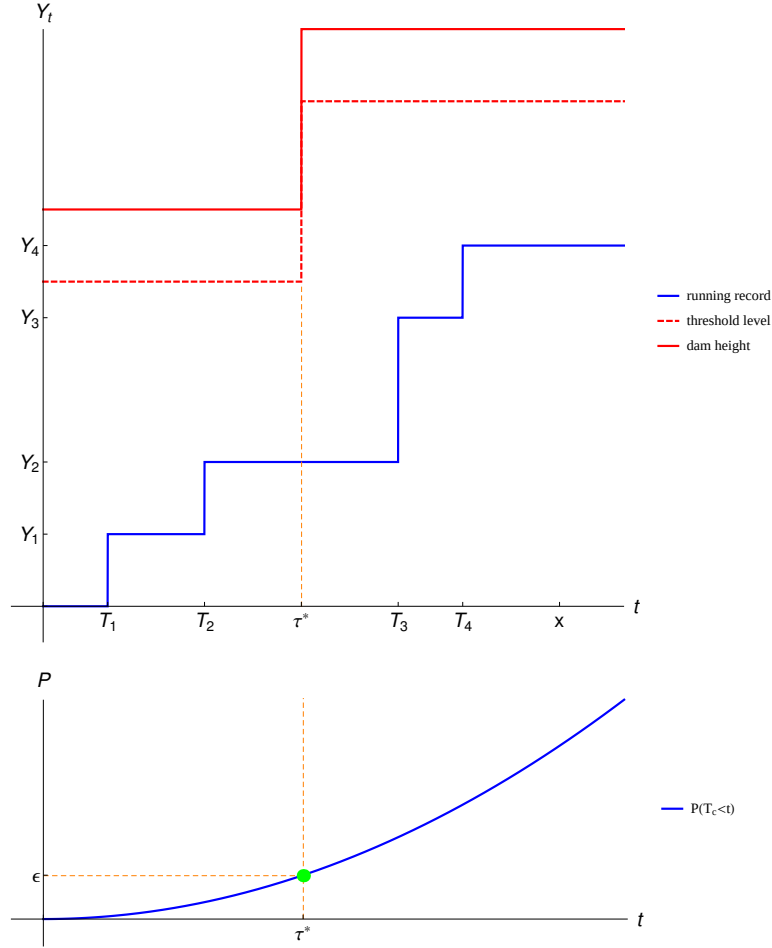
Figure 7: A probabilistic strategy of dam management incorporating an early warning signalling for water releases based on the exceedance probability P(T_c < t) .
