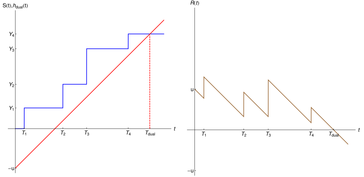
Figure 2: Model B. Left panel: h_{\text{dual}}(t) (red/straight line) represents the lower risk level bound and S(t) (blue/staircase line) is the stochastic gain process. Right panel: the risk process R(t) .
