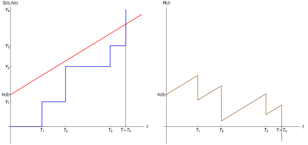
Figure 1: Model A. Left panel: h(t) (red/straight line) represents the deterministic upper critical level and S(t) (blue/staircase line) is the stochastic loss process. Right panel: the risk process R(t) .
