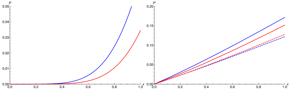
Figure 5: The probabilities P(T_c < x) (solid lines) and P(T_c < x, Y > H - h) (dashed lines) against varying x . Left panel: exponential water inflow severities with parameter values \lambda = 10 and \alpha = 0.2 . Right panel: Pareto water inflow severities with parameter values \lambda = 1 , \beta = 50 and \theta = 2 . Other parameter values: H = 100 , h_1 = 0.8H (blue lines) and h_2 = 0.9H (red lines).
