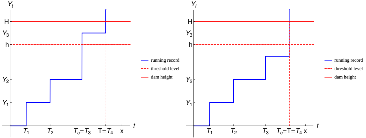
Figure 4: A stochastic model for the risk of overtopping.
