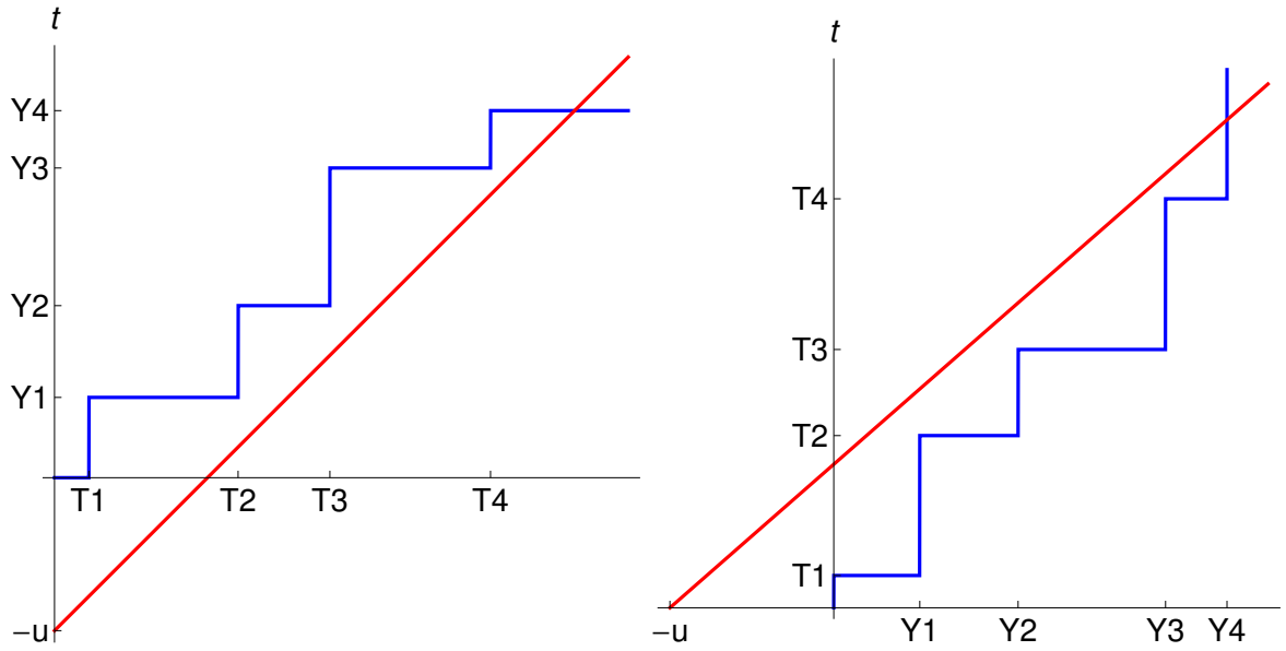
Figure 3: A connection between model A and model B through a reflection along the 45^\circ line.
