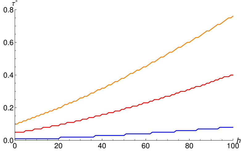
Figure 8: Alarm times against varying threshold levels. Blue, red and orange lines represent \epsilon = 0.01, 0.05, 0.1 respectively. Parameter values: \lambda = 1 , \beta = 50 , \theta = 2 and H = 100 .
