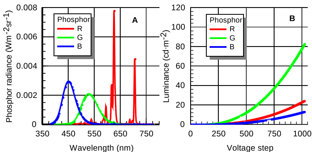
Figure 3-3: Absolute spectral radiance measurement for the red (R), green (G) and blue (B) phosphors of the CRT display (A) and luminance versus gun voltage calibration for the R, G and B phosphors (B).
