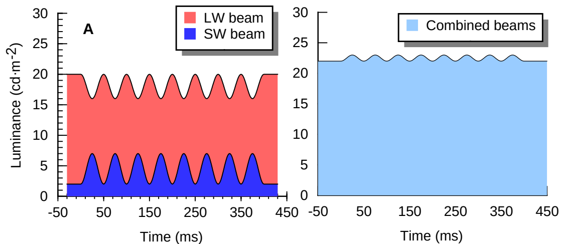
Figure 3-5: Temporal profiles of the luminances of the MAP test beams. The LW and SW beams are modulated sinusoidally in counter phase (A) and combine to the residual modulation profile of the flickering stimulus (B).
