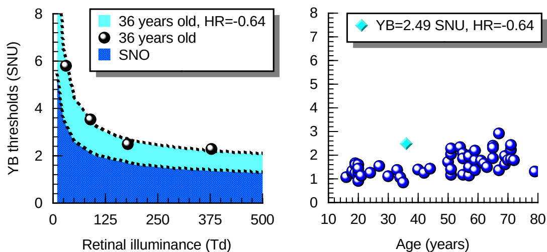
Figure 5-7: A 36-year-old subject with an abnormal HR index.
