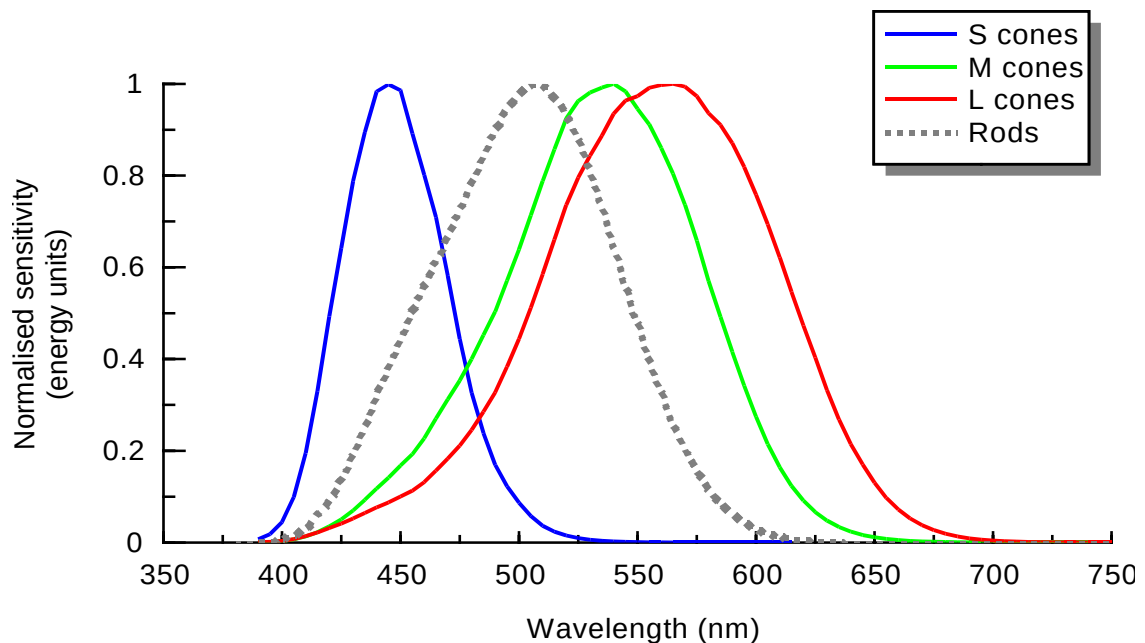
Figure 2-1: Fundamental cone and rod spectral sensitivities (Stockman and Sharpe, 2000). S cones show maximum sensitivity at ~445 nm, rods at ~507 nm, M cones at ~540 nm and L cones at ~ 565 nm (data obtained from http://www.cvrl.org/ ).
