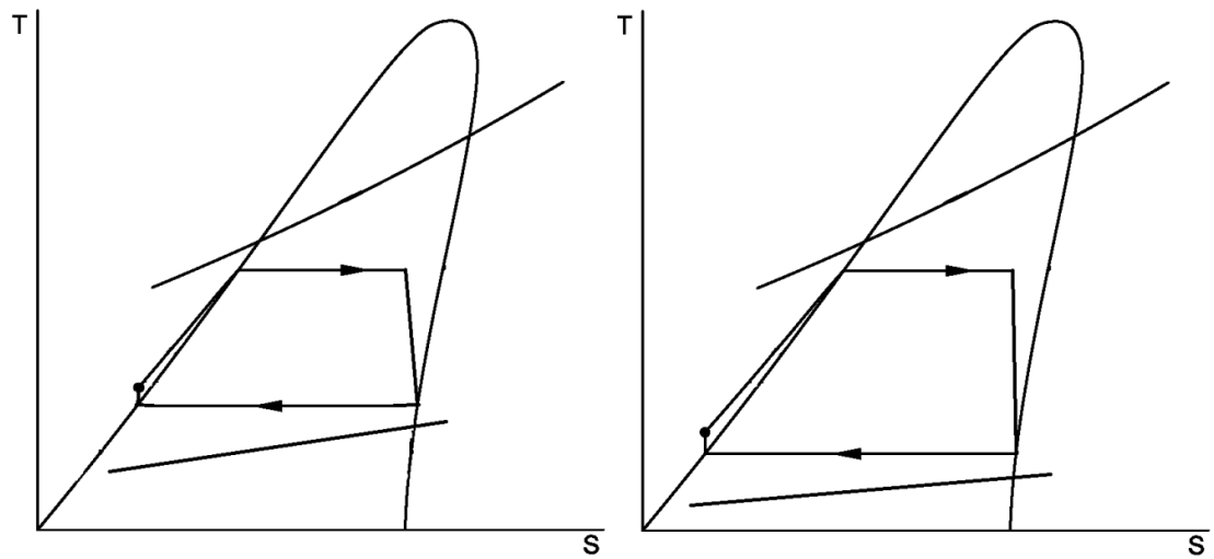
Figure 54 T-s diagram illustrating the effect of reducing condensing temperature with fixed waste heat
