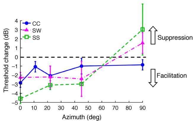
Figure 3. Variation of the target detection threshold (measured without pedestal) with the deviation of the flankers from the collinear axis for three observers: CC (blue), SW (magenta), and SS (green). Note that the facilitatory effect of the flankers has a broad location tuning over azimuth.
