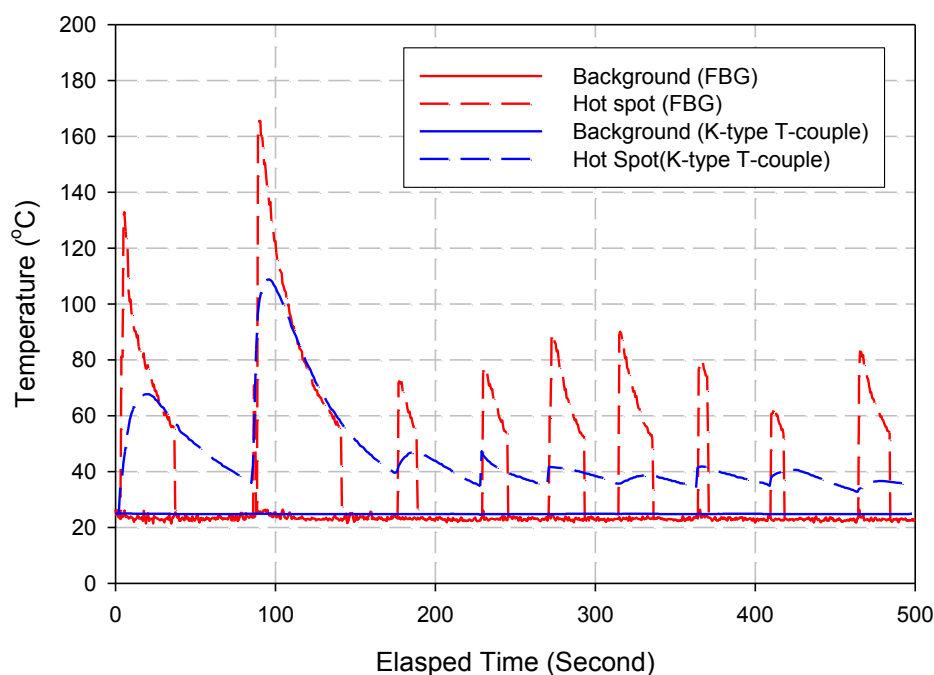
Figure 6.9: Response of FBG-based fire alarm system to hot spot compared to that of the K-type thermocouple
