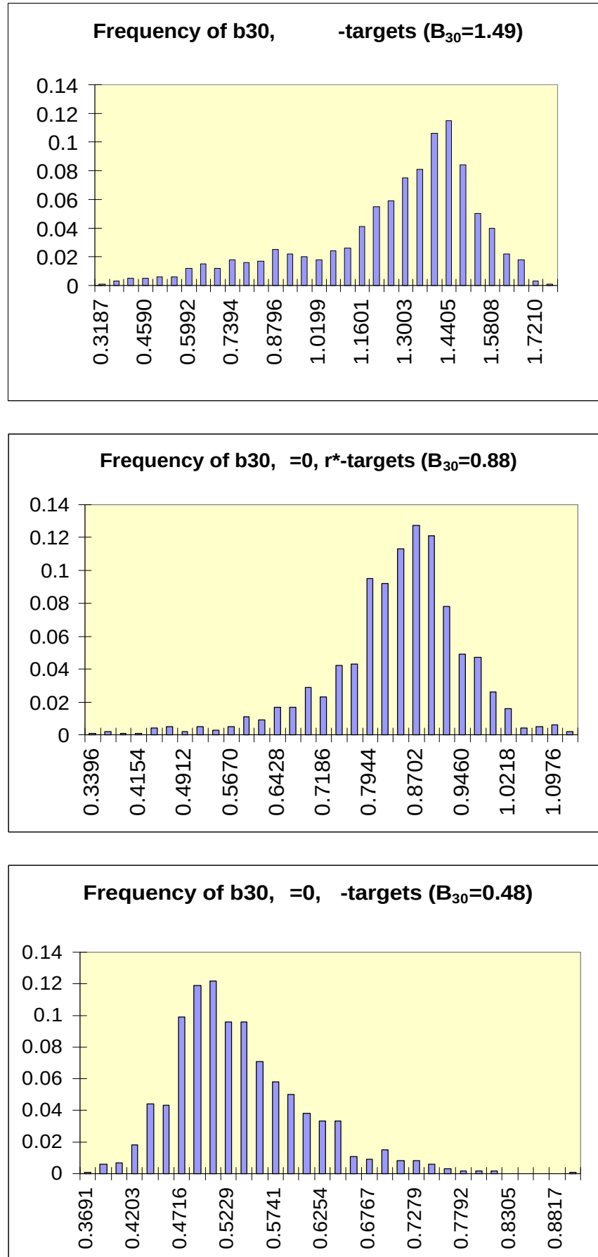
FIGURE 11: DISTRIBUTIONS OF b_{30}
