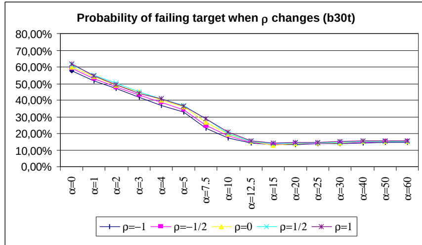
FIGURE 10: RISK MEASURES WHEN \rho CHANGES (b30t)
