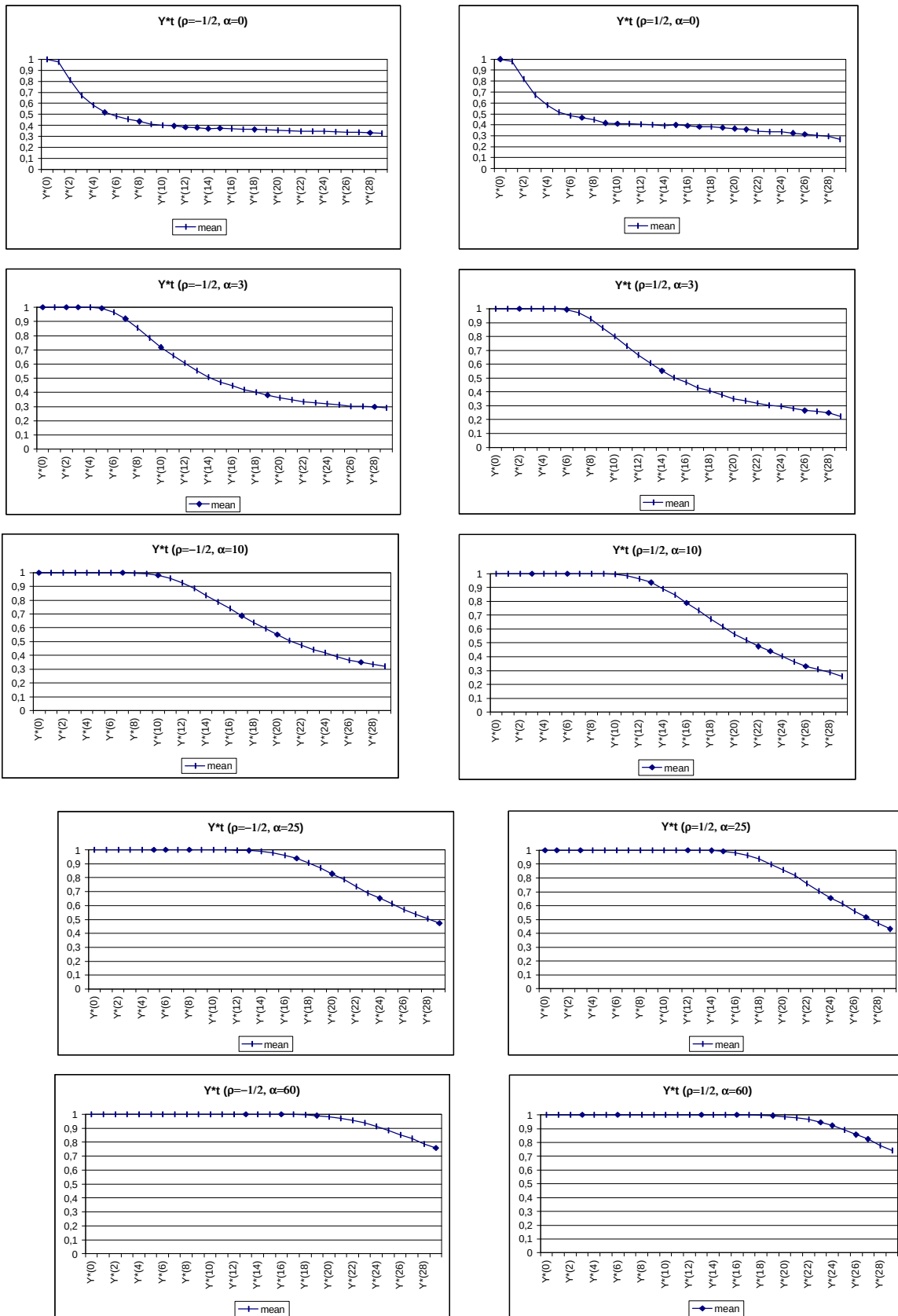
FIGURE 2: CHANGING DISUTILITY FUNCTION (THE VALUE OF \alpha )
