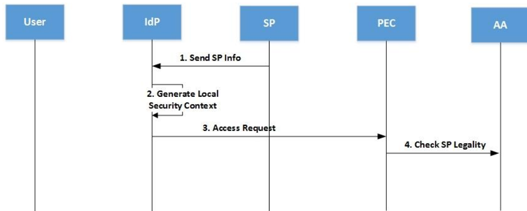
Figure 5.6Authenticaiton for SP
