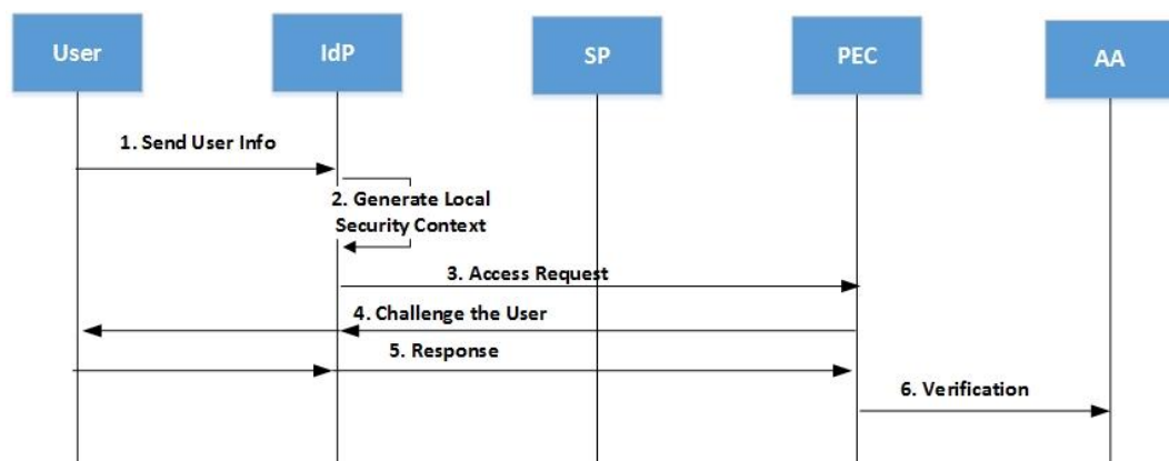
Figure 5.7Authentication for User
