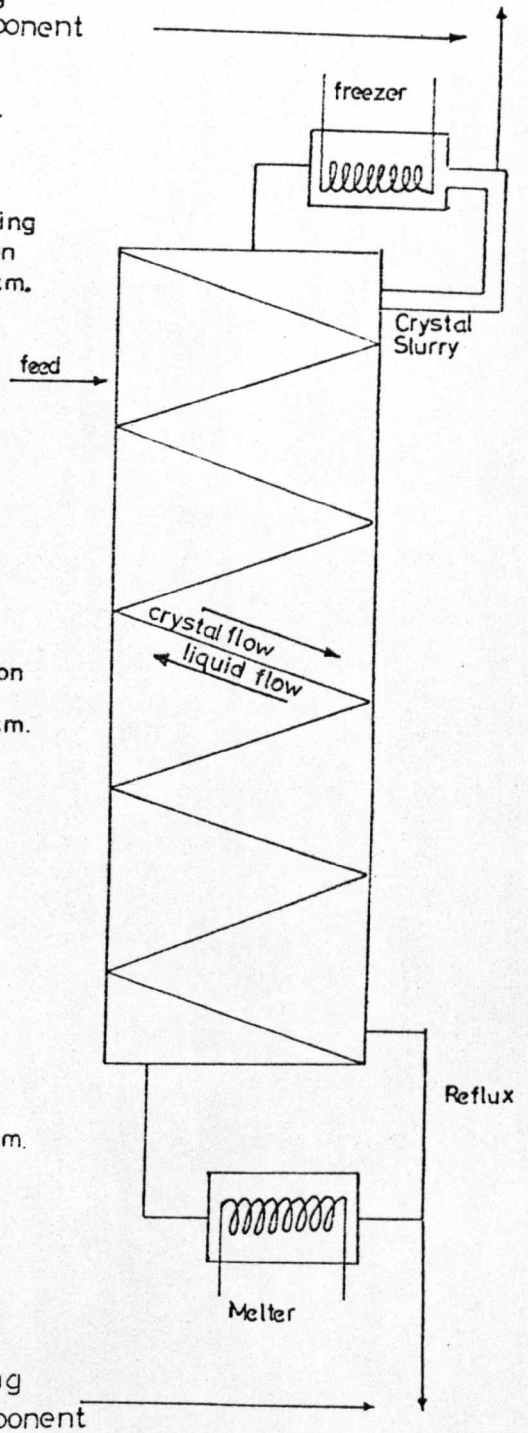
FIG.2 FLOW DIAGRAM
