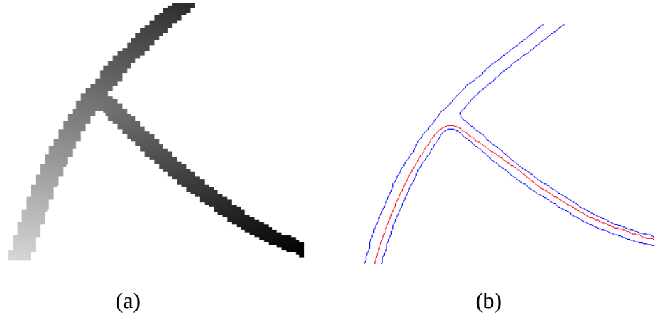
Figure 2.1: Illustration of the ‘hugging corner’ effect [22] in a synthetic image. (a) The distance map, (b) The centreline (shown in red) is extracted through the application of Dijkstra searching algorithm based on the distance field in (a). The centreline is attracted to the boundaries of the object (in blue) at sharp turn positions.
