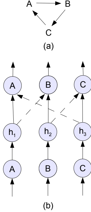
Figure 3: (a) An example of a cyclic argumentation network and (b) its neural implementation whose parallel computation produces, in a single pass through the network, a terminal state [-1, -1, -1] with no prevailing argument, following a grounded argumentation semantics
