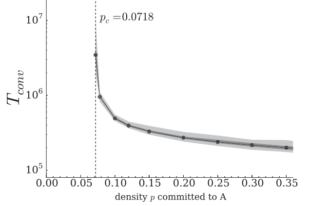
FIG. 1. Numerical results for convergence time T_{conv} in the binary NG with a randomly selected committed minority for a population of N = 10^4 agents. Only two opinions are possible: A or B, with a state of consensus reached when everyone knows only opinion A. Committed agents begin with knowledge of A and introduce this new opinion to the rest of the population who initially know opinion B. The median of 100 simulations show that convergence time diverges at the analytically derived critical threshold of p_c \approx 0.0718 . The 95% and 50% confidence intervals are shown shaded in dark and light grey.
