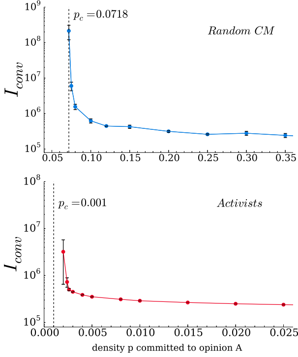
FIG. 2. (Color online) Average number of interactions required to reach convergence I_{conv} vs p in the NG in activity driven networks for a population of N = 10^4 agents for 100 simulations (Top). I_{conv} diverges at the same p_c for random committed minorities as in systems with homogenous activity distributions (Figure 1). (Bottom) Activists (commitment correlated with high probability to speak) on the other hand show considerable advantage in needing fewer interactions to reach consensus and a numerical threshold of p_c \approx 2 \times 10^{-3} , agreeing well with the analytically derived p_c \approx 1 \times 10^{-3} .
