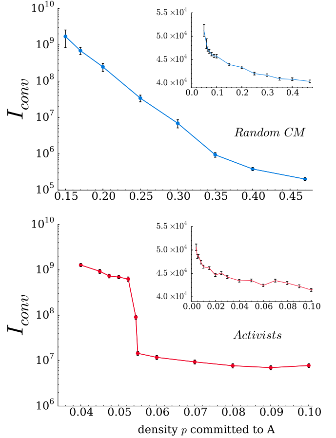
FIG. 4. (Color online) I_{conv} in the NG on a real network of N = 1222 agents containing two weakly connected communities vs a random rewiring of the network (inset). Agents begin with knowledge of opinion A or B dependent upon the community they are originally a part of with a select group in community A remaining committed to A . I_{conv} is the number of interactions at which 95% or more of the network agrees upon opinion A . In both the original community based network and the rewired network, shown in the insets, activists (bottom) show considerable advantage over randomly selected committed minorities (top) in needing fewer committed agents.
