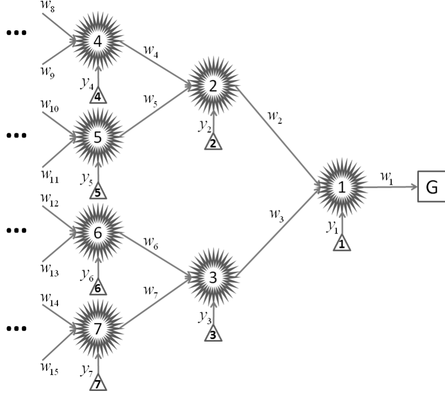
Figure 3: The structure of a half binary tree.
