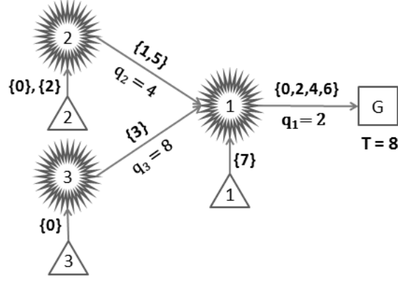
Figure 4: An optimal PPS with q_1 = 2 for Example 2, specified by its link activation times.
