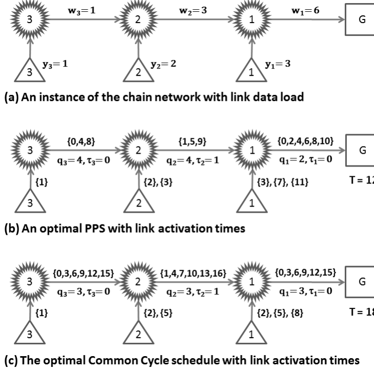
Figure 2: The chain network and its schedules for Example 1.
