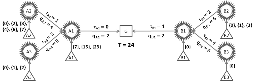
(a) An optimal PPS with its periodicity and initial link activation time
