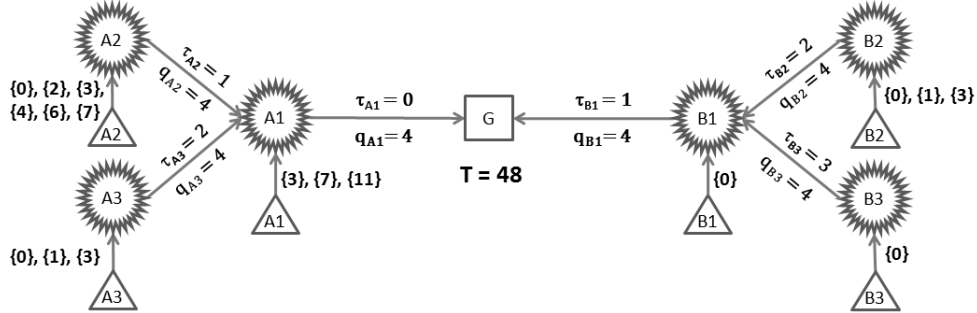
(b) The optimal Common Cycle schedule with its periodicity and initial link activation time
