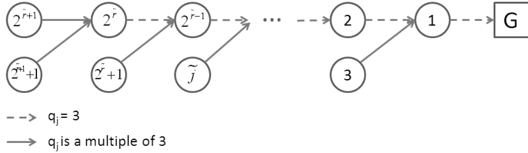
Figure 5: Illustration of J_2 subnetwork part of a feasible solution with q_1 = 3 .
