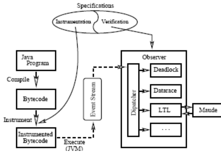
Figure 2-8 – The JPaX architecture [75]
