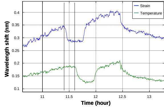
Fig. 11. Example of time lag between strain and temperature sensors.
