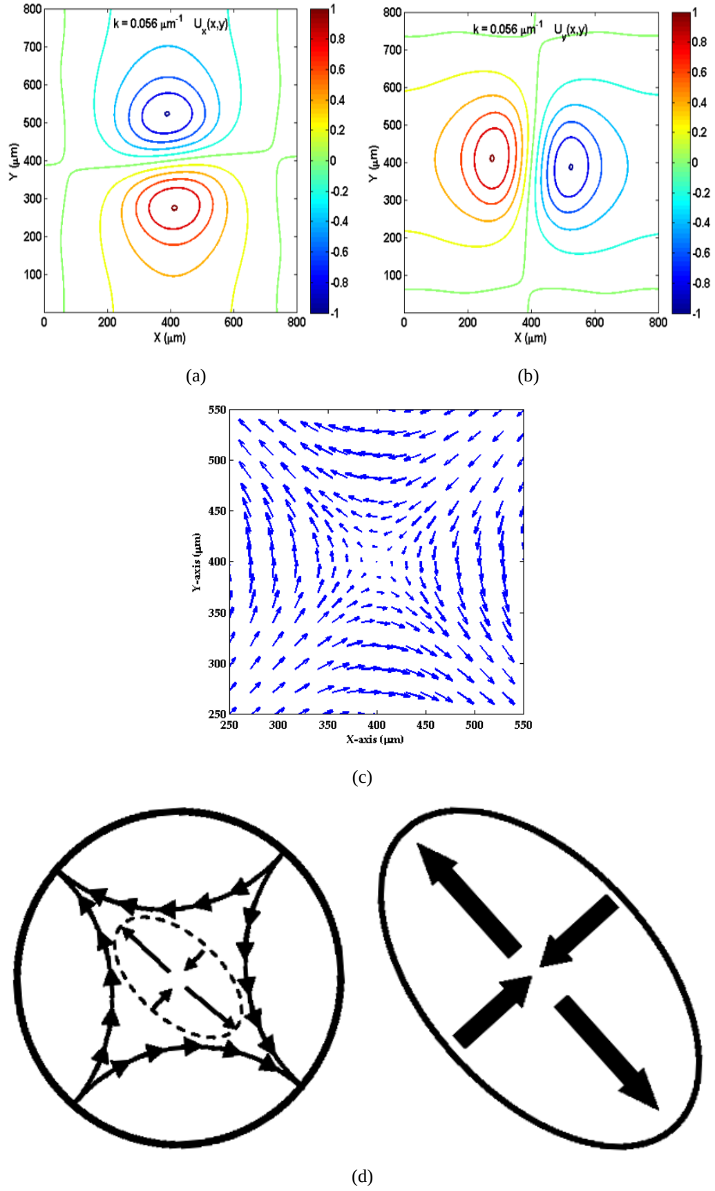
Figure 4.6. Torsional-Radial mode (a) U_x and (b) U_y displacement (c) vector U_t plot and (d) the periodic displacement of Torsional-Radial at fa=5.838 \mu\text{m}.\text{GHz} .
