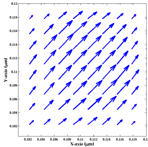
Figure 3.12. The vector displacement fields U_t = \bar{U}_x + \bar{U}_y of the acoustic waveguide of the bending mode at k = 200 \text{ m}^{-1} .
