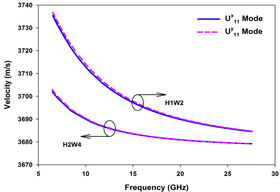
Figure 5.1. The variation of acoustic wave velocities with the acoustic frequencies for H1W2 and H2W4 waveguides.
