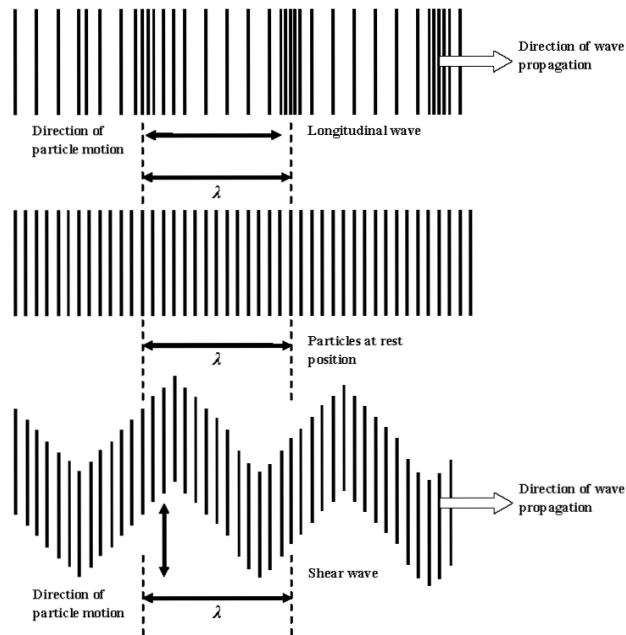
Figure 2.7. Longitudinal and shear wave direction of propagation.
