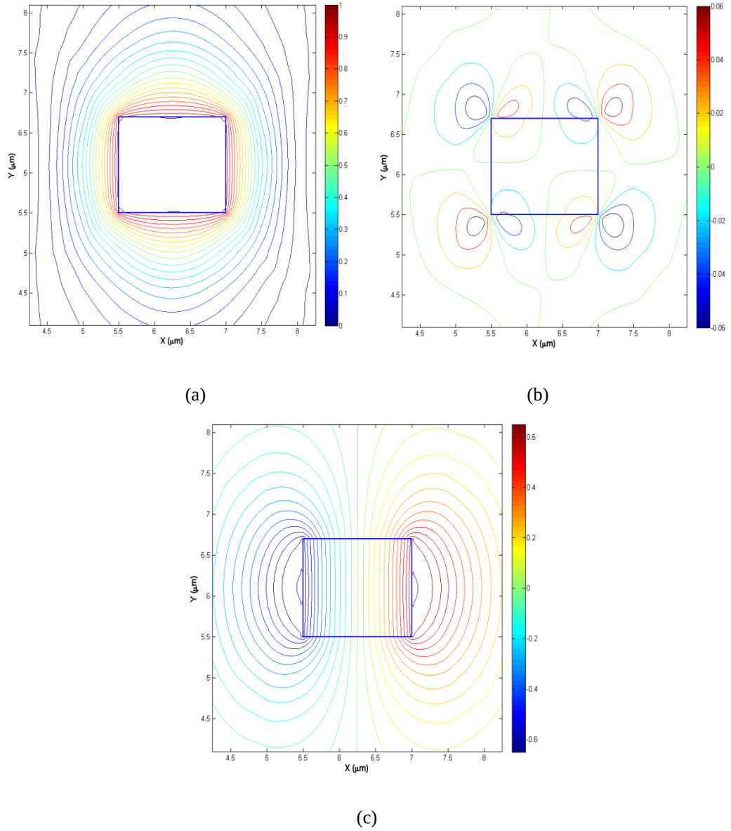
Figure 5.20 The U_{11}^x Bending mode (B2) at k_0 = 1.5 \mu m^{-1} of (a) U_x , (b) U_y and (c) U_z displacement vector.
