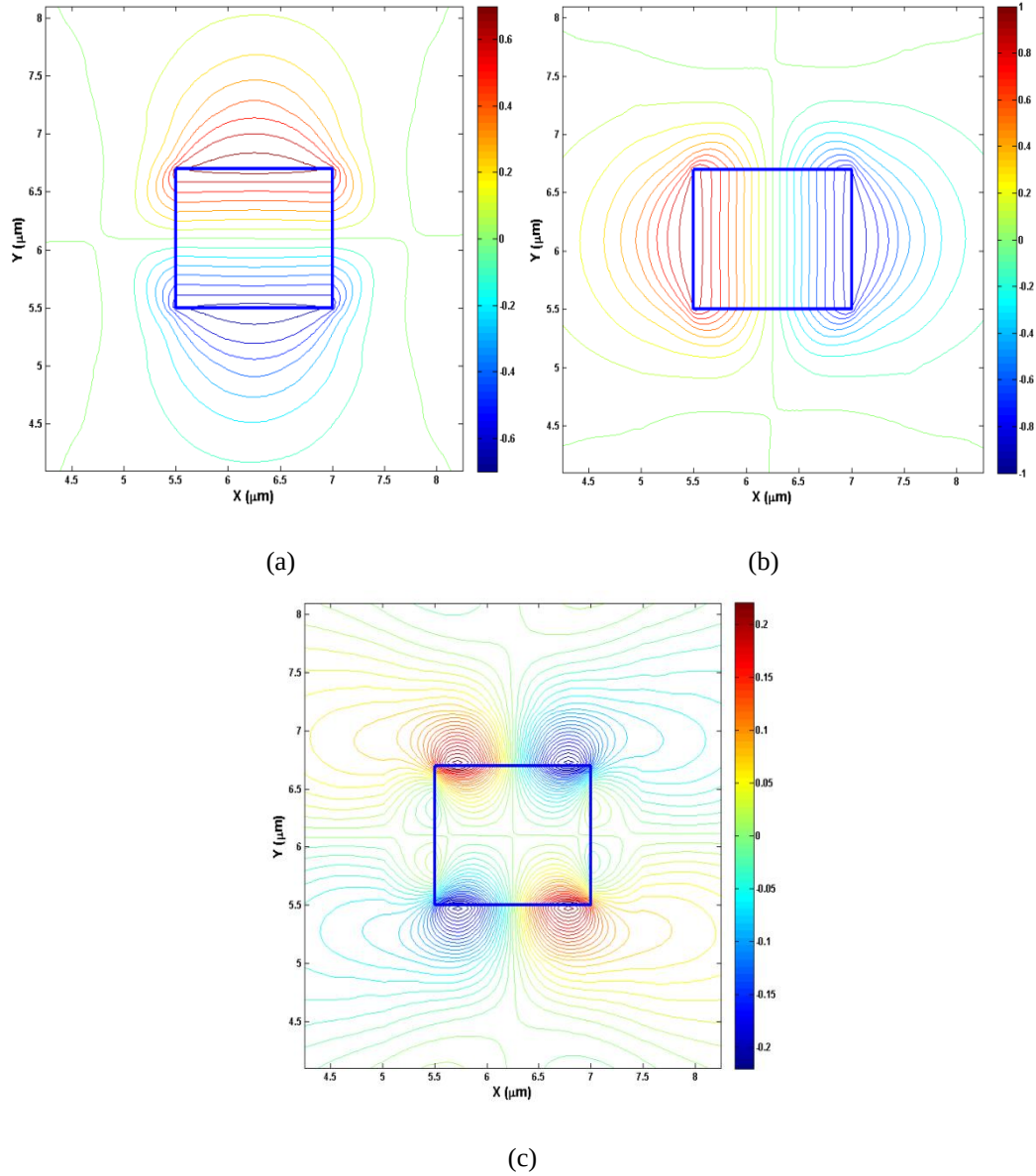
Figure 5.27. Displacement vector profiles (a) U_x (b) U_y , and (c) U_z of the T1 U_{21}^y mode at k=1.5 \mu\text{m}^{-1} .
