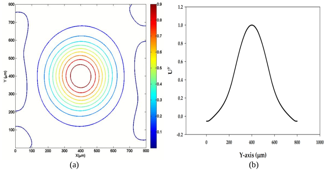
Figure 4.3. The S_{01} mode (a) the U_y contour plots (b) its line plot at fa=5.18 \mu m.GHz of the transverse S_{01} mode.
