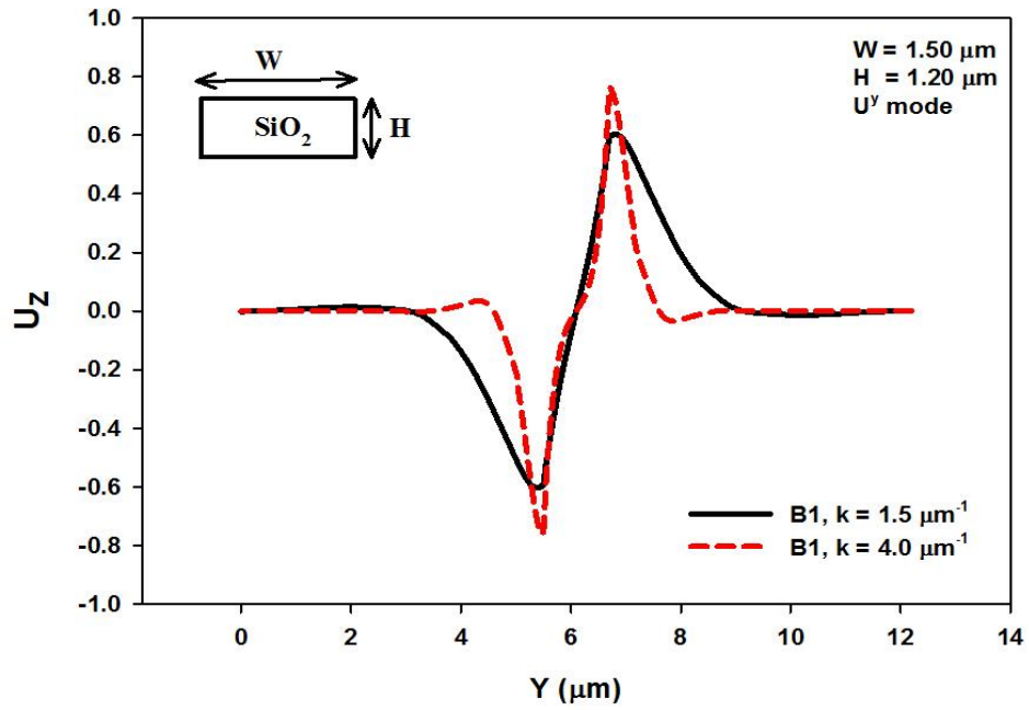
Figure 5.26. Variation of U_z along y-axis of the B1 mode( U^y ) at k = 1.5 \mu\text{m}^{-1} and k = 4.0 \mu\text{m}^{-1} .
