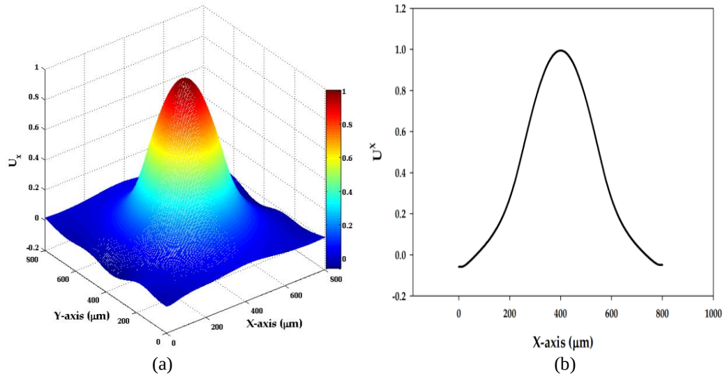
Figure 4.2. The transverse S_{01} mode for (a) the 3-D plot and (b) 2-D plot of the U_x at fa=5.18 \mu m.GHz .
