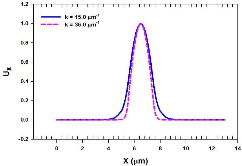
Figure 5.3. Variation of the U_x displacement vector of the U_{11}^x mode along the x -axis at k=15 \mu\text{m}^{-1} and k=36 \mu\text{m}^{-1} .
