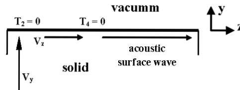
Figure 2.8. Configuration for acoustic surface wave analysis.
