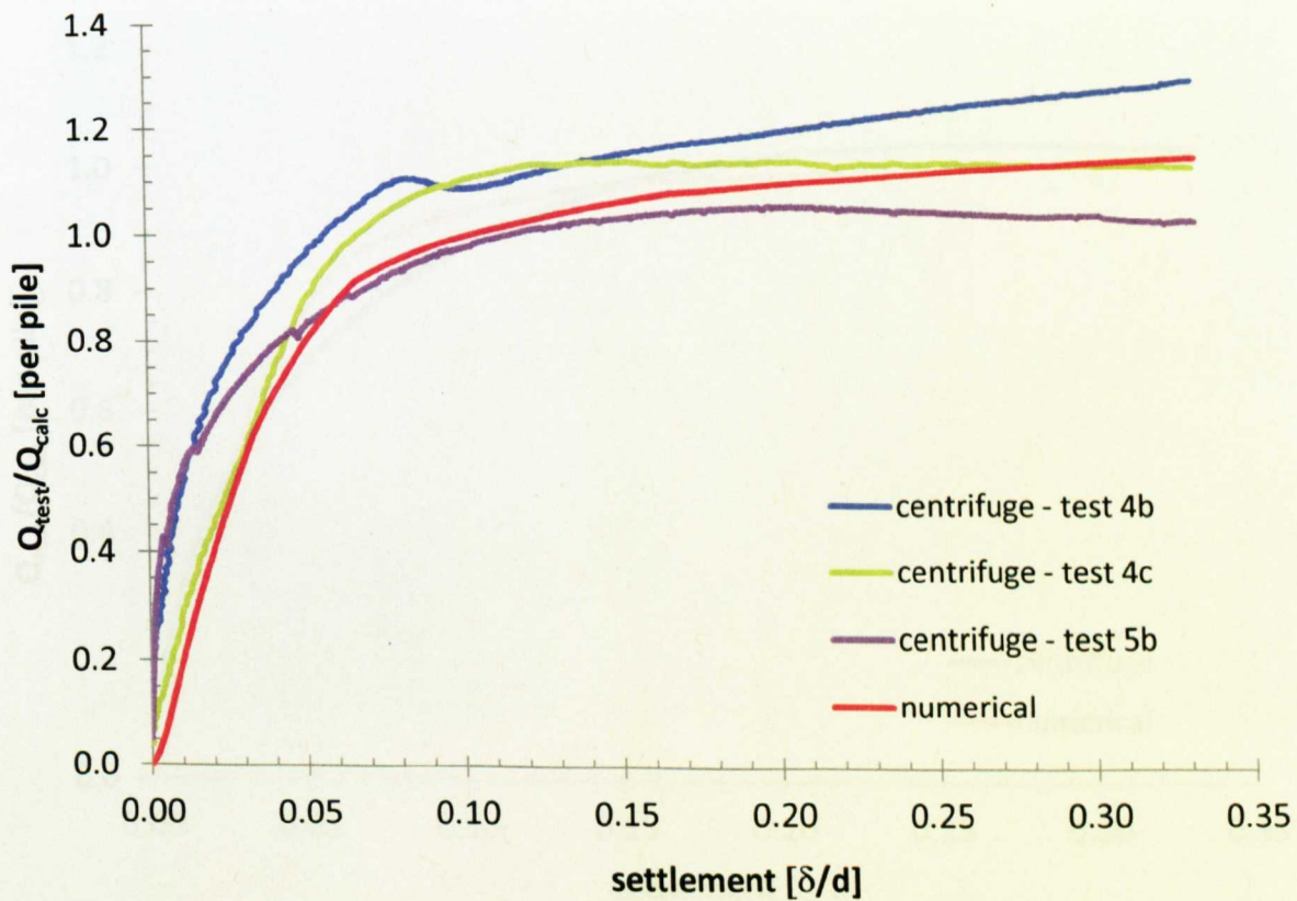
Figure 8.08 Q_{test}/Q_{calc} vs settlement comparison: TS16_2.00
