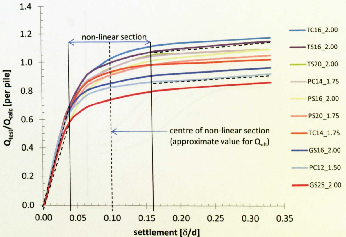
Figure 8.27 Efficiency vs settlement: numerical modelling
