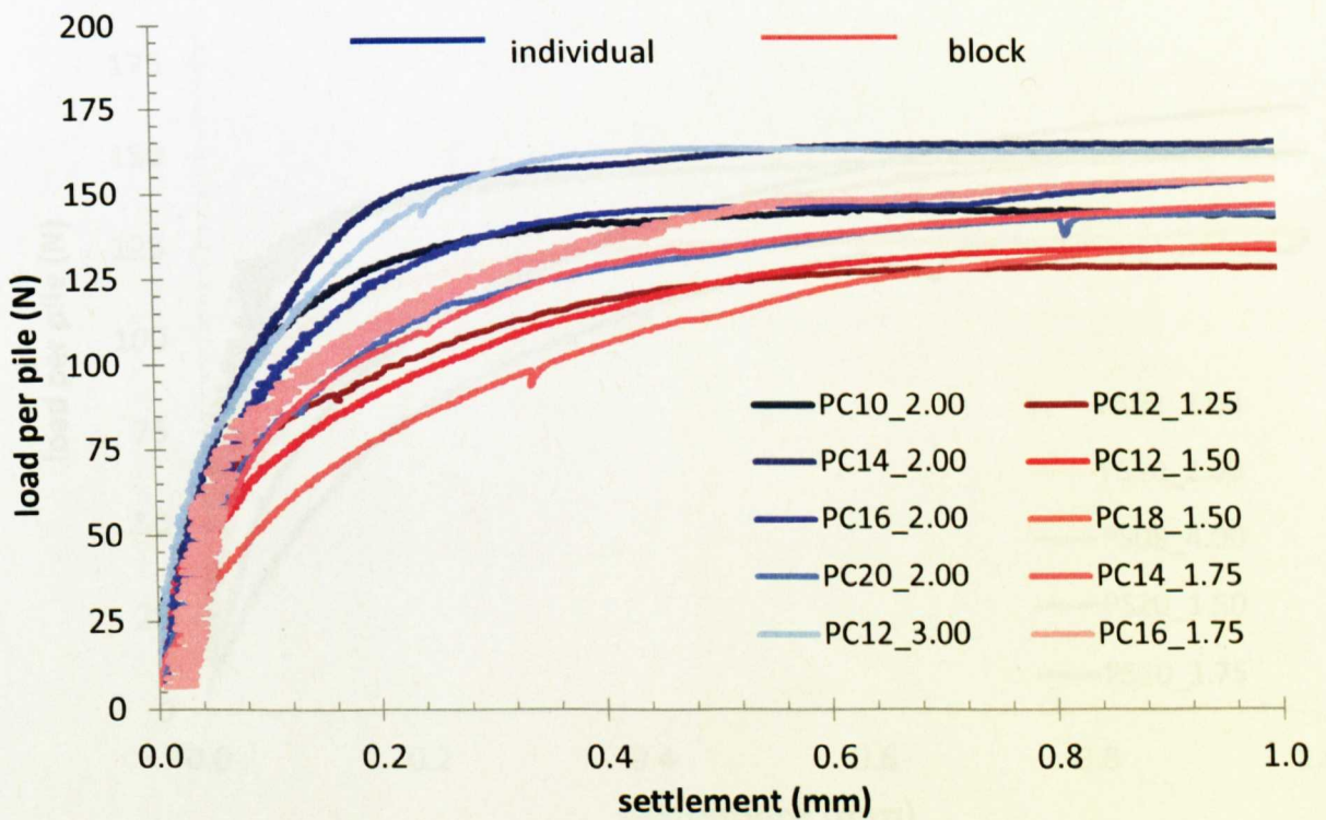
Figure 6.13 Load vs settlement: individual/block comparison - perimeter groups (circular)
