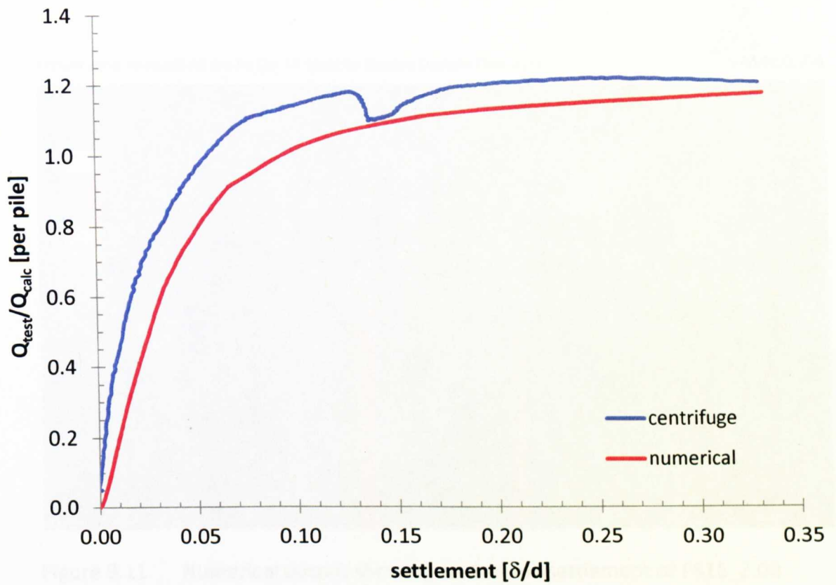
Figure 8.09 Q_{test}/Q_{calc} vs settlement comparison: TC16_2.00
