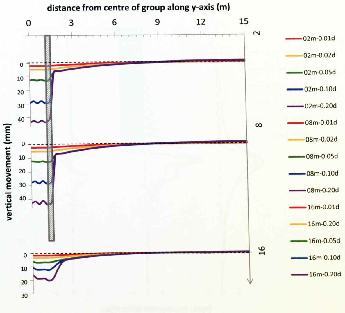
Figure 8.23 Vertical soil movement change with settlement ( sp_A )
