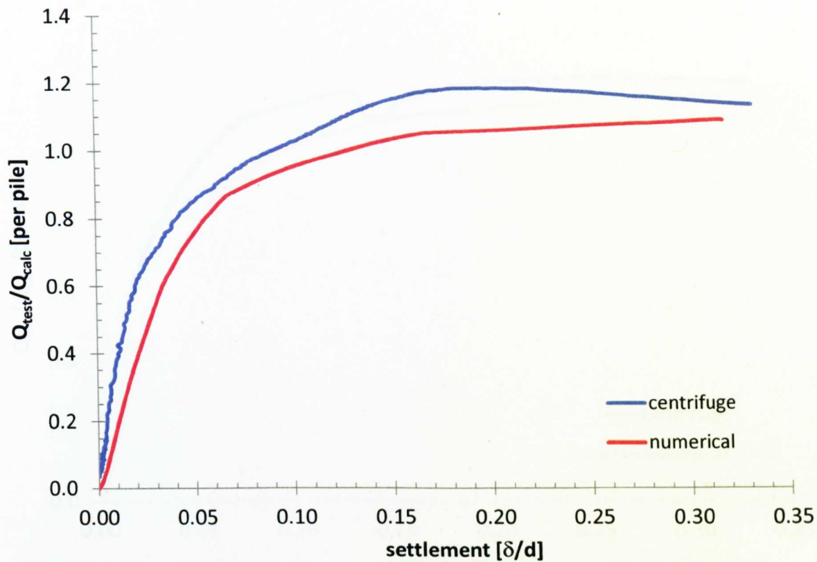
Figure 8.07 Q_{test}/Q_{calc} vs settlement comparison: TS20_2.00
