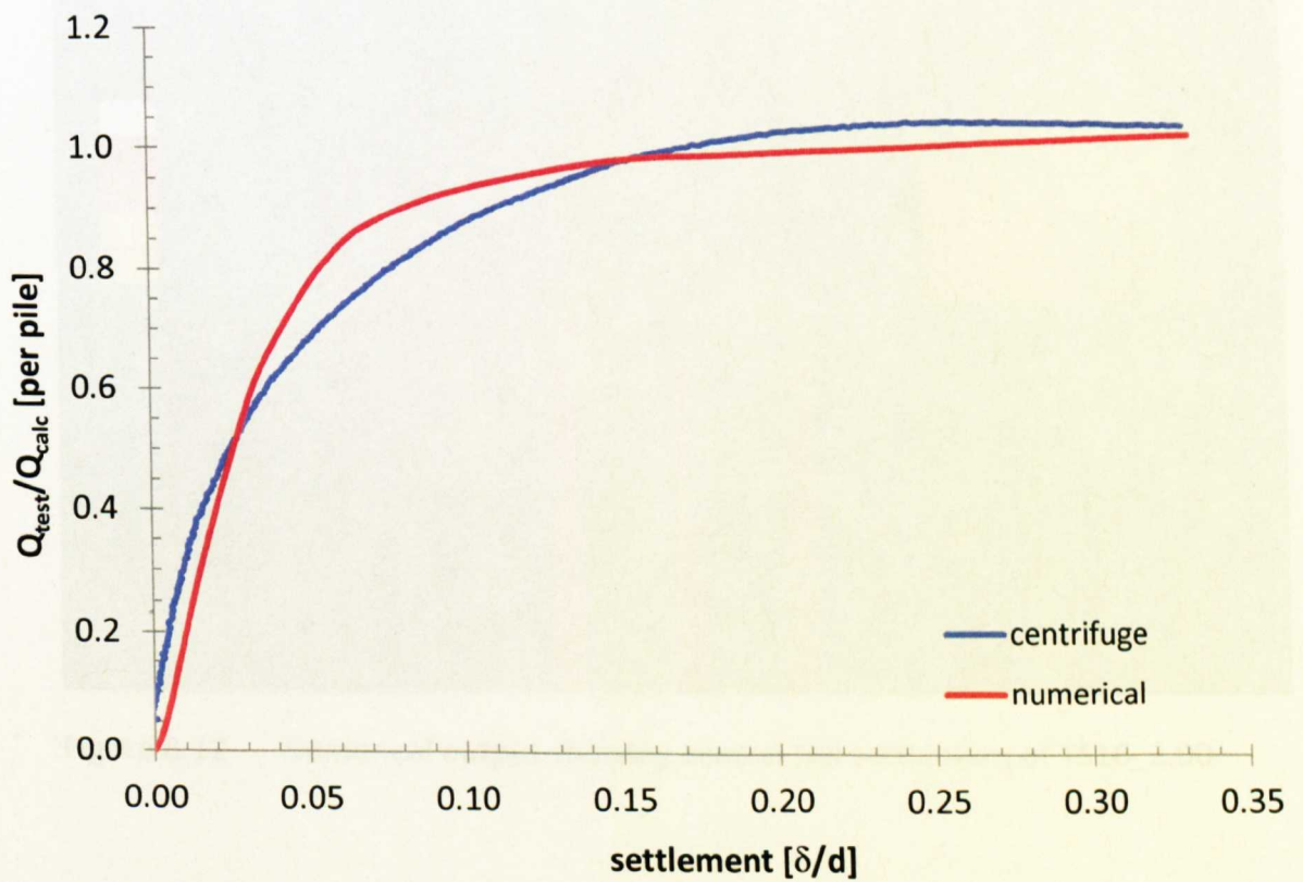
Figure 8.10 Q_{test}/Q_{calc} vs settlement comparison: TC14_1.75
