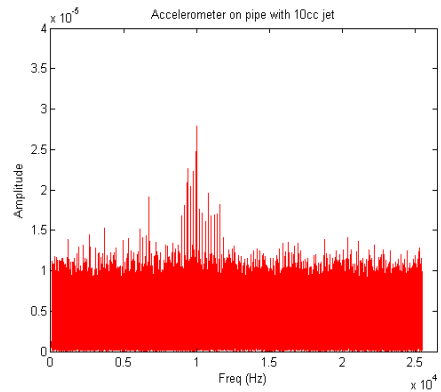
Figure 7.21 Accelerometer on pipe with addition of noise (SNR=12dB)
