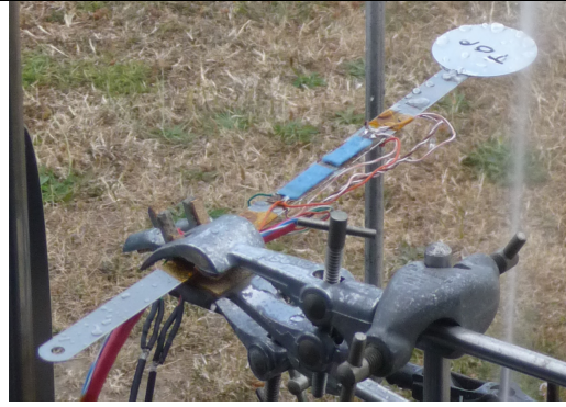
Figure 6.7 Deflecting strain gauge, directly on steam
