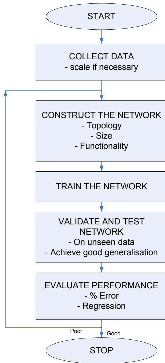
Figure 3.2 ANN Iteration Cycle
