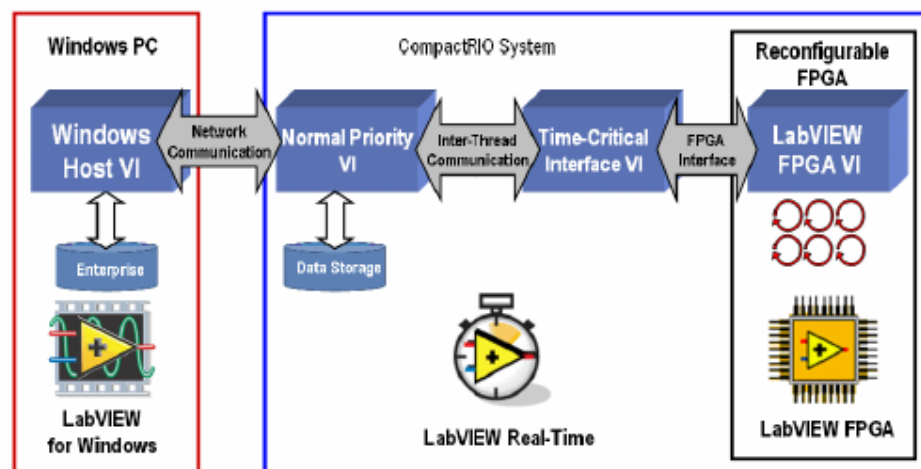
Figure 6.2 Labview block diagram for data communication, National Instruments (2009b)
