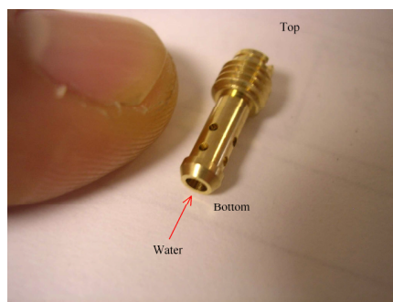
Figure 4.2 Carburettor jet
