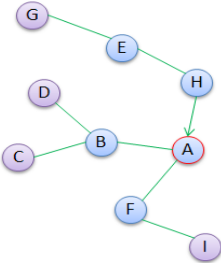
Figure 7-8: After receiving finish discovery message from all children, sink node adds its own ID to message paths and figures out a polygon.
