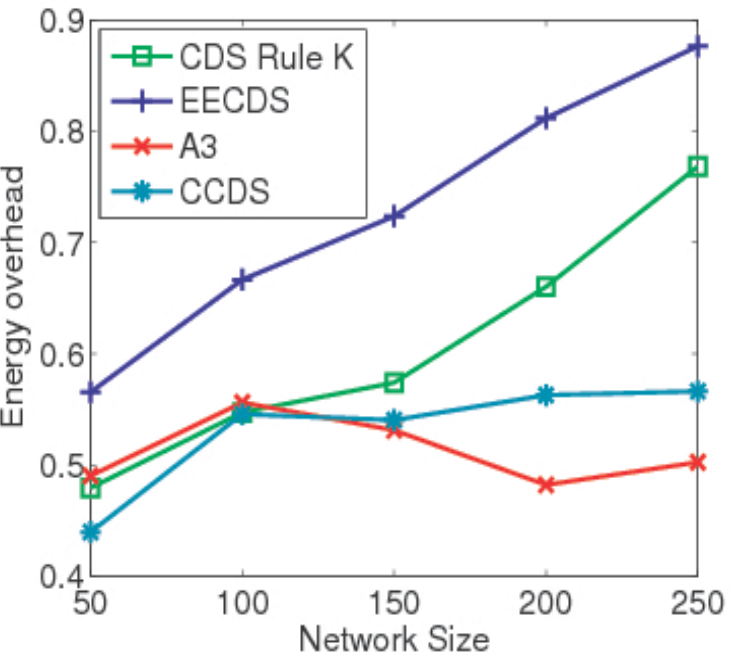
Figure 5-11: Energy overhead under topology maintenance.
