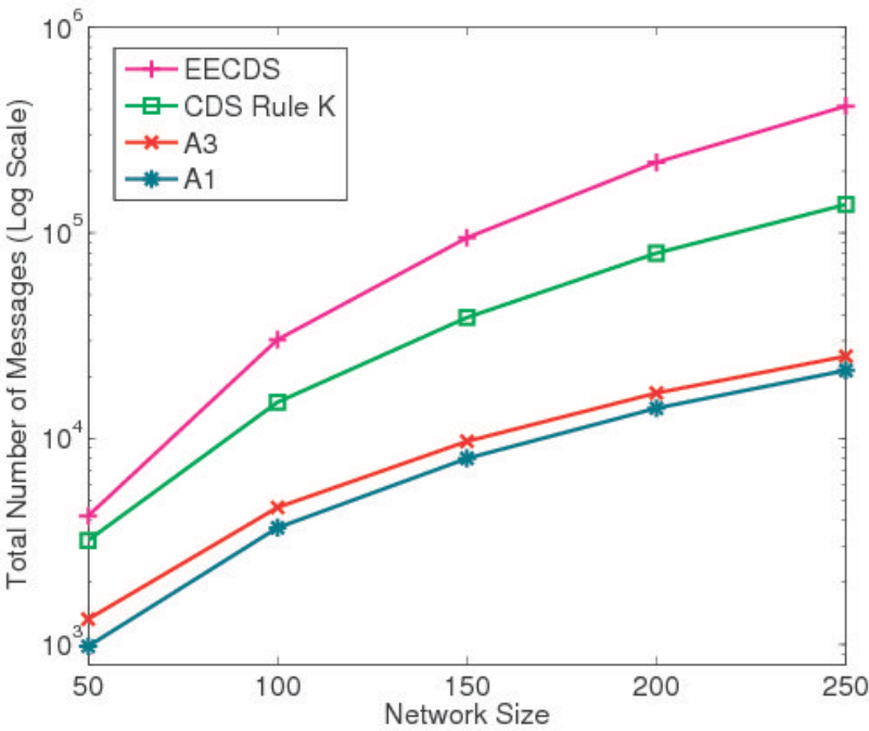
Figure 6-7: Message overhead under varying network size.
