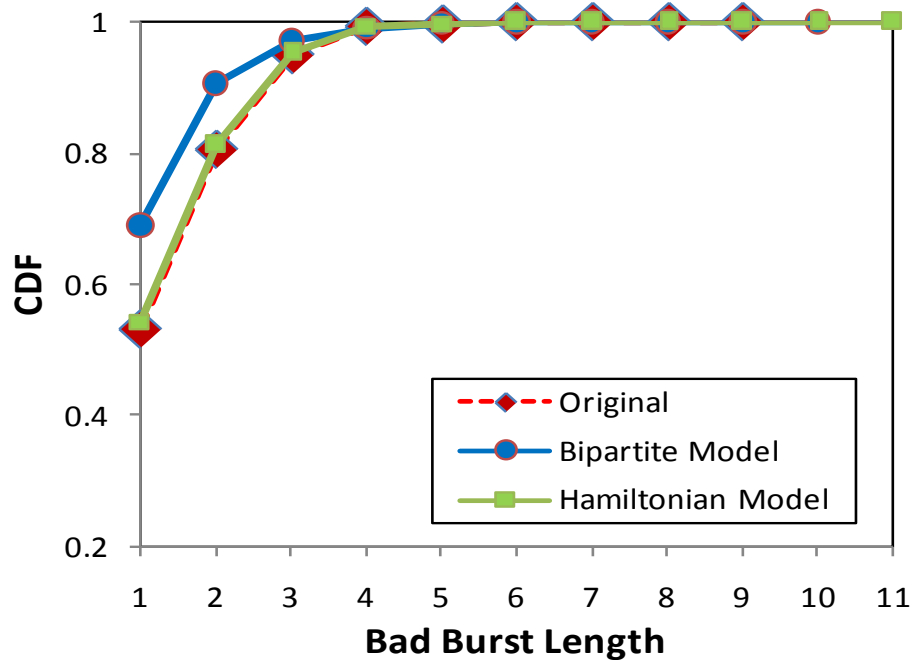
Figure 3-11: Bad burst length distribution for 802.15.4 bit error traces at K = 8 .
