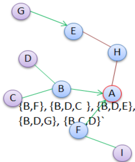
Figure 7-7: Node B extends the message paths with its own ID and sends it to its parent node. Message paths sent by B are shown in the figure.
