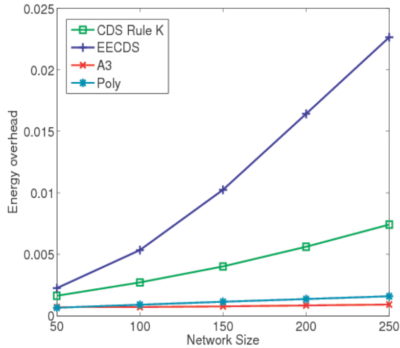
Figure 7-15: Energy overhead when node densities are varied.
