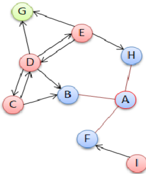
Figure 7-4: Next level nodes again broadcast the Hello message after changing the parent IDs to their respective parent.
