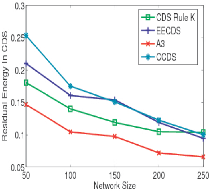
Figure 5-10: Residual energy in CDS under topology maintenance.
