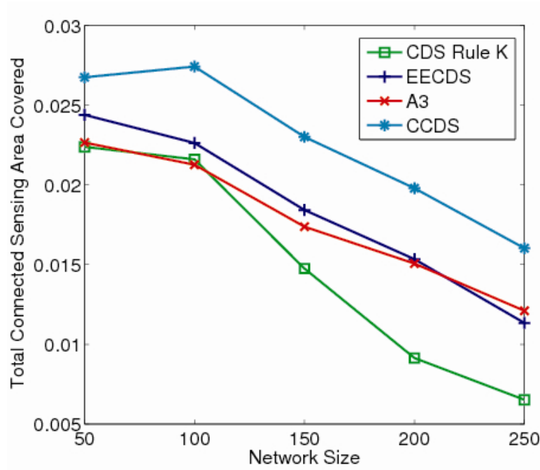
Figure 5-17: Total area of sensing coverage.
