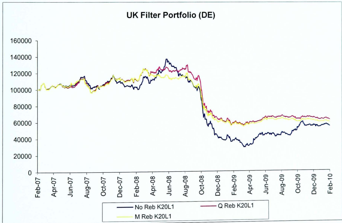
Figure 5-8: Out-of-sample performance of the UK Filter portfolio; \lambda=1 , with maximum 20 stocks in the basket, under the three rebalancing frequencies as selected by the DE.
