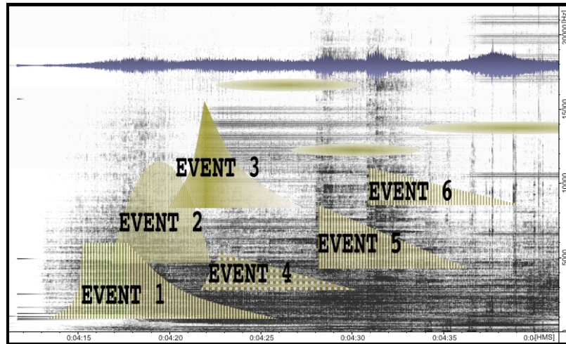
Fig. 4.14 Event chains.
