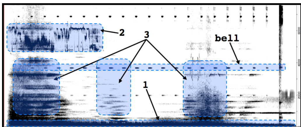
Fig. 4.24 Four timescales.
