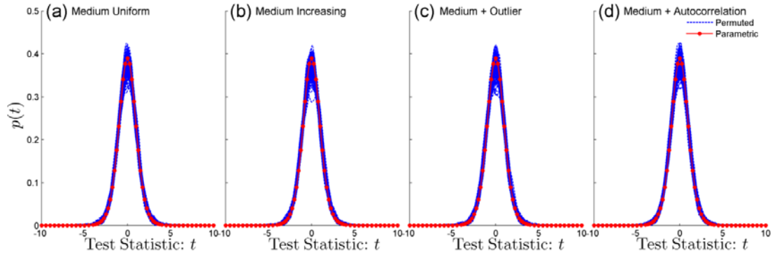
Figure 3.8 Two-hundred randomly sampled permutation distributions of OLS linear regression test-statistics with the parametric Student's t-distribution (11 degrees of freedom) overlaid for 4 scenarios of noise pattern: (a) medium uniform noise, (b) medium increasing noise, (c) medium noise with an outlier and (d) medium noise with autocorrelation. These distributions are for stable simulated series hyperbolic measurement noise at 13 th RA measurement (6 years). The average p-value for the two-sample Kolmogorov-Smirnov test is for (a) 0.52, (b) 0.50, (c) 0.53 and (d) 0.54.
