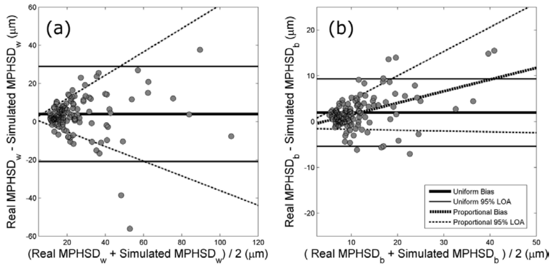
Figure 5.2 Bland-Altman plots showing series-wise, agreements between (a) average within examination MPHSD ( \text{MPHSD}_w ) for real and simulated mean topography data and (b) agreement of between examination ( \text{MPHSD}_b ) for real and simulated mean topography data. The mean difference (bias) of average \text{MPHSD}_w is 3.5\mu\text{m} (95% limits of agreement: -20.9\mu\text{m} to 28.8\mu\text{m} ). The mean difference of \text{MPHSD}_b is 2.0\mu\text{m} (95% limits of agreement (LoA): -5.4\mu\text{m} to 9.3\mu\text{m} ). Uniform 95% LoA illustrate only approximate limits of agreement as heteroscedasticity of this data is apparent. Dashed lines indicate statistically significant linear proportional bias for \text{MPHSD}_b and the significant linear proportional increase of the widths of the 95% LoA for \text{MPHSD}_w and for \text{MPHSD}_b .
