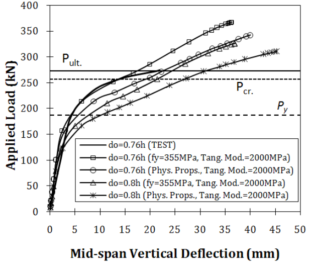
Fig. 6: Load-deflection curves
