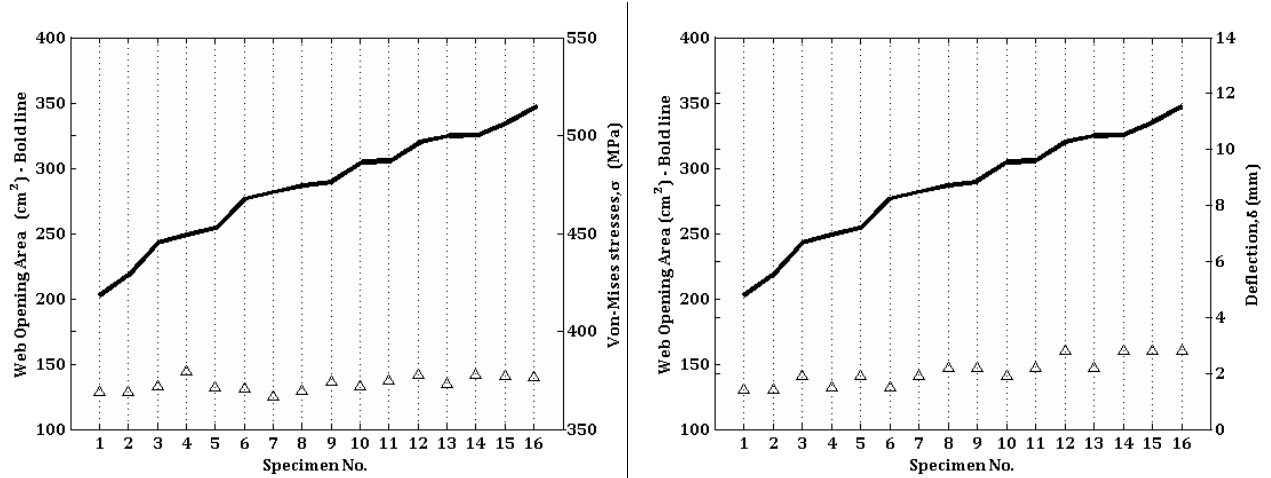
Fig. 9: Von-Mises nodal stresses (left) and maximum vertical deflections (right) at P_y
