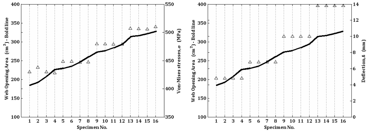
Fig. 14: Von-Mises nodal stresses (left) and maximum vertical deflections (right) at P_{ult} .
