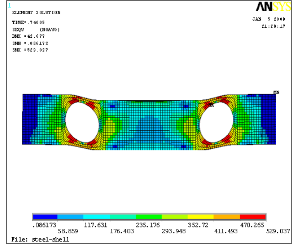
Fig. 8: Von-Mises stresses at failure load
