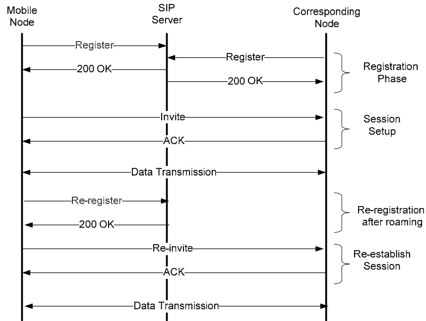
Figure 2-3: SIP signalling
