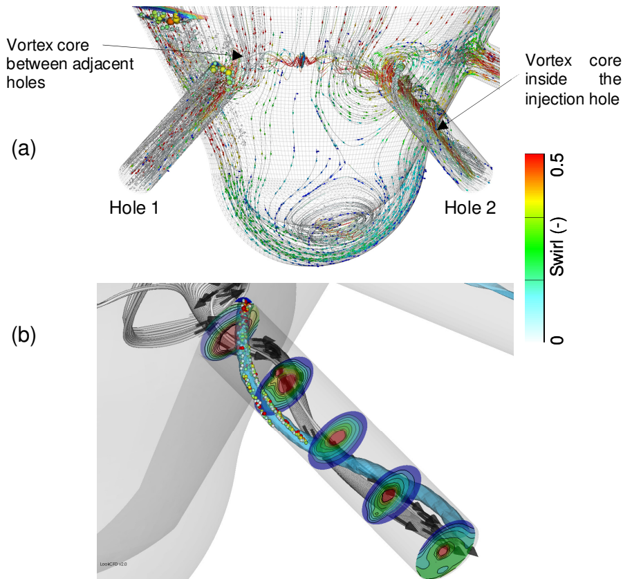
Figure 7-8: Model predictions for the original VCO nozzle using slightly eccentric needle position. Calculations indicate (a) formation of a strong vortex formed in-between adjacent holes and (b) the vortex core inside the injection hole can be linked with the area where string cavitation has been observed. (by courtesy of [164])
