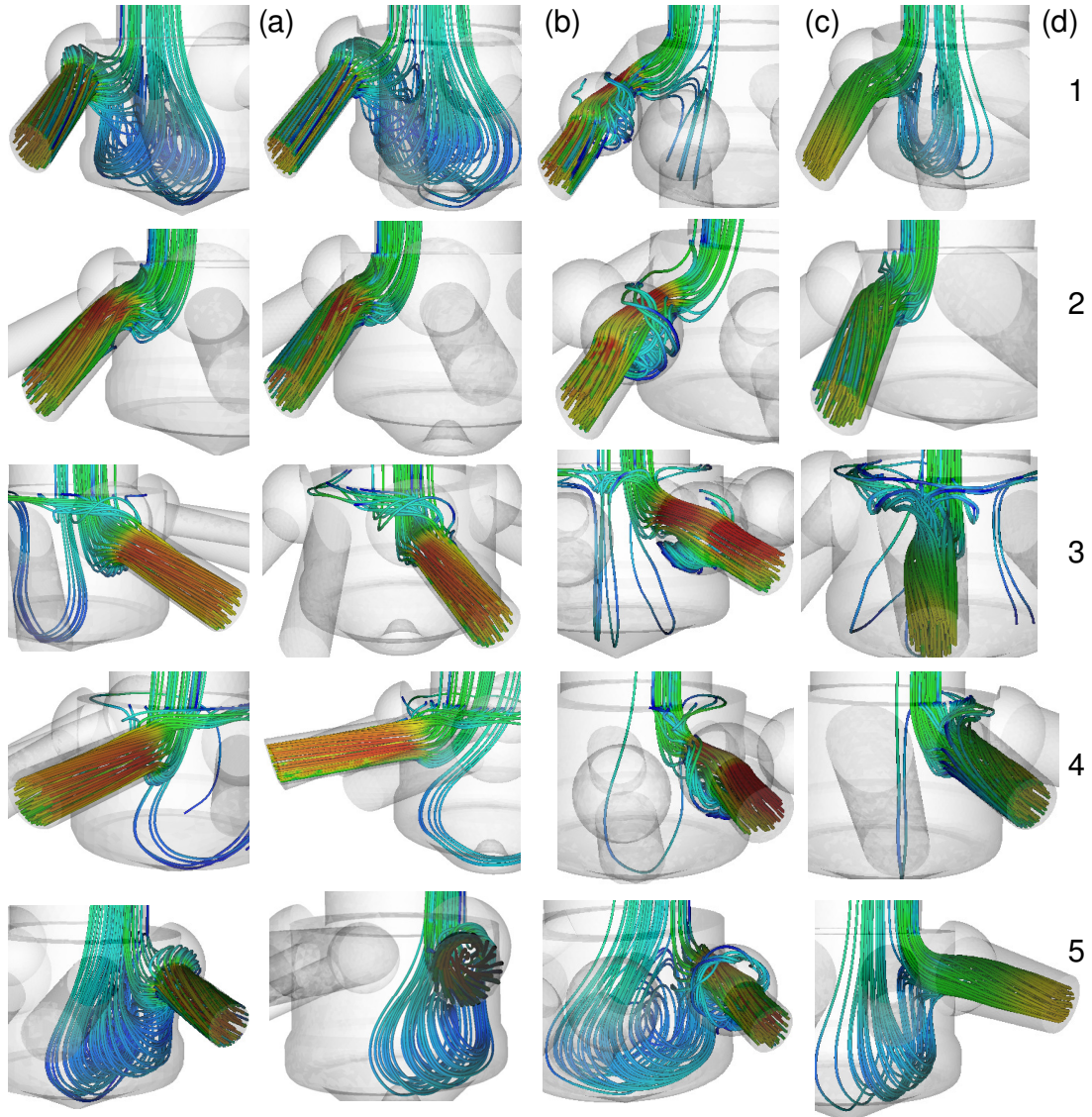
Figure 4-41: Predicted flow structure inside the nozzle volume. Standard (a), Modified Sac Volume (b), Middle-hole spheres (c) and Taped Holes (d) Designs.(2)
