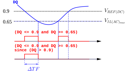
Fig. 3. Falling slew region and \Delta TF
