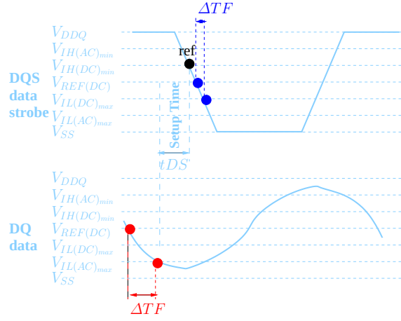
Fig. 4. Relation between the reference point and the corresponding \Delta TF of DQ and DQS
