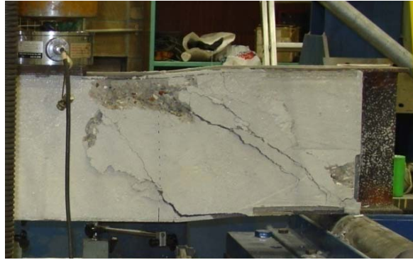
Figure 8. USFB No.2 at Failure point.
