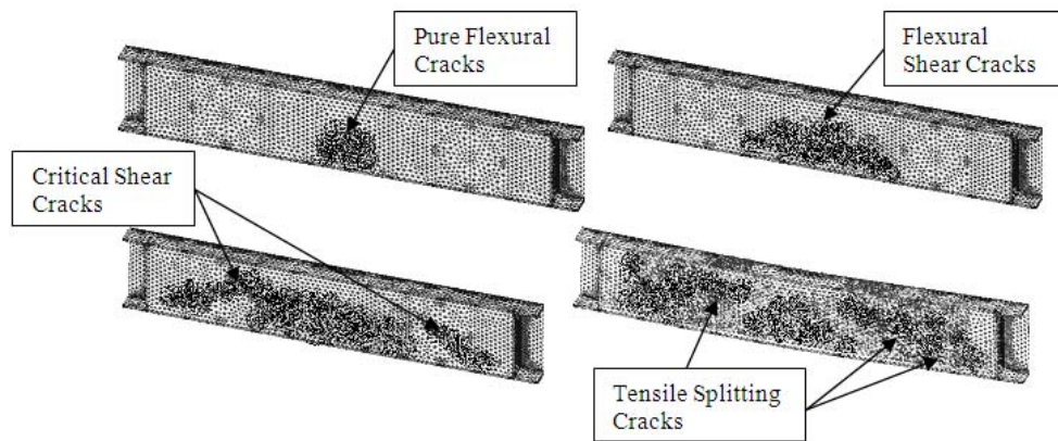
Figure 5. Bending and shear crack development at the front side of the beam.
