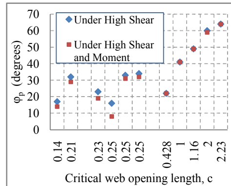
Figure 5: \phi_p values of the first plastic hinge
