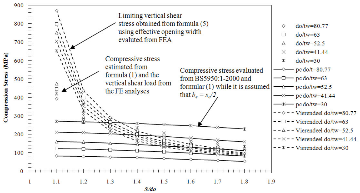
Fig. 11: Compressive strength of the 'strut' compared with FE failure stress (A1 & B1)
