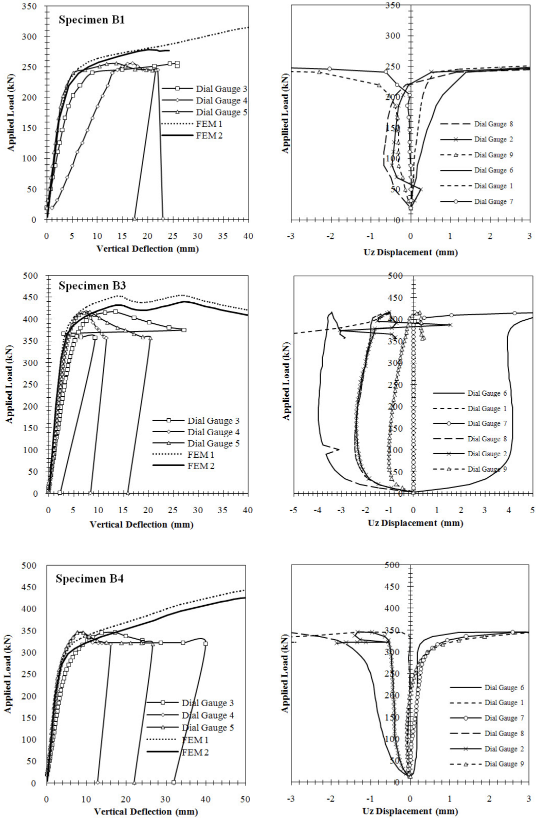
Fig. 3: Comparison of experimental and FEM extracted results
