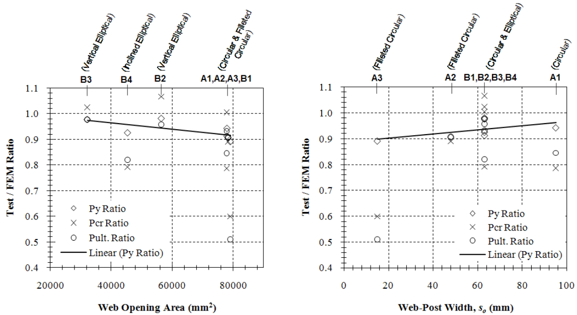
Fig. 5: Variations of test loads to FEM loads
