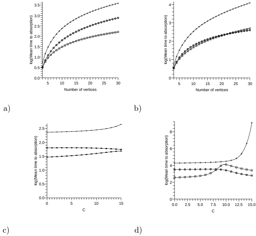
Figure 5. Comparison of the mean time to absorption when a mutant Hawk invades into a resident population of Doves between a star (crosses), a circle (circles) and a complete graph (boxes) in the Hawk-Dove game with payoff matrix 3.1 in the case where (a) C = 2 , (b) C = 13 and the number of vertices varies, (c) the number of vertices is equal to 10 and C varies, (d) the number of vertices is equal to 60 and C varies.
