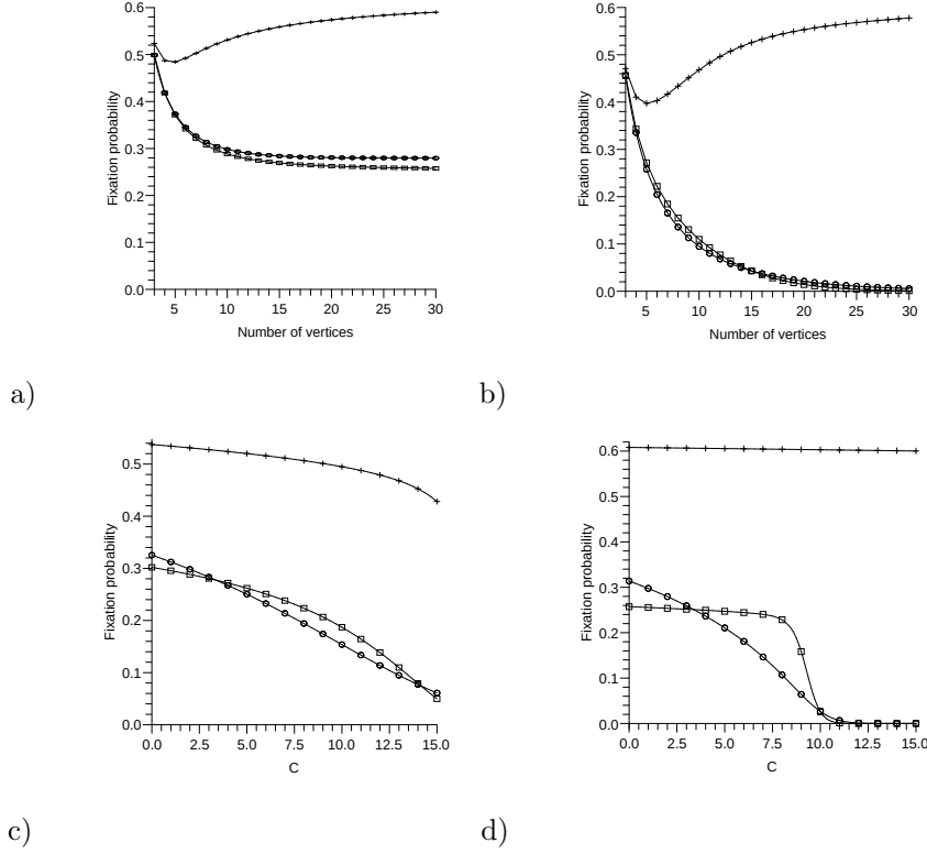
Figure 3. Comparison of the fixation probability of a mutant Hawk when it invades into a resident population of Doves between a star (crosses), a circle (circles) and a complete graph (boxes) in the Hawk-Dove game with payoff matrix 3.1 in the case where (a) C = 2 , (b) C = 13 and the number of vertices varies, (c) the number of vertices is equal to 10 and C varies, (d) the number of vertices is equal to 60 and C varies.
